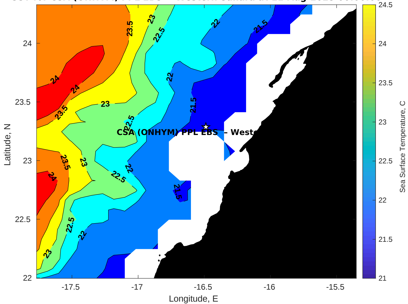
SST for CSA (ONHYM) PPL EBS - Western Sahara at 11-Aug-2025 00:00:00
