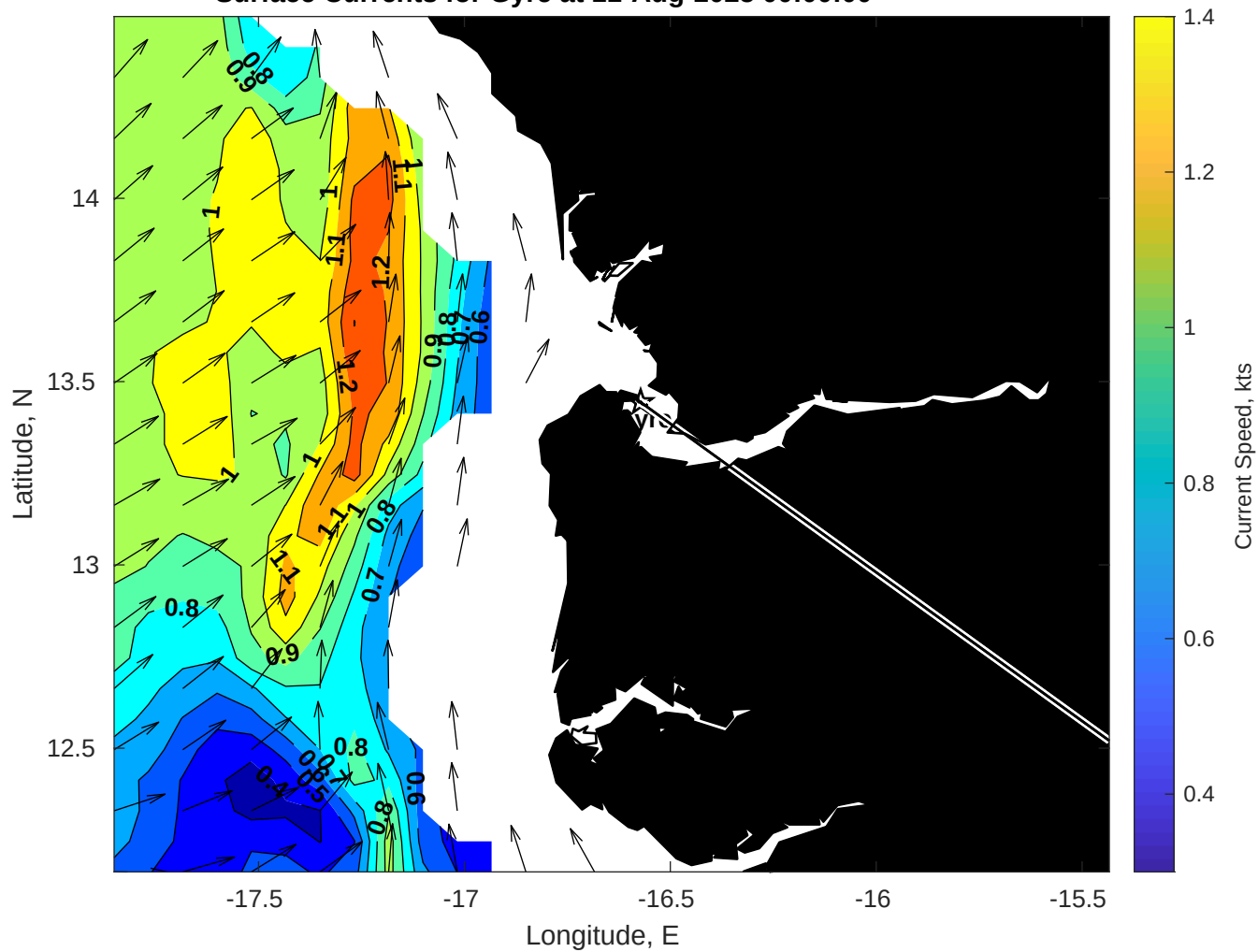
Surface Currents for Gyre at 11-Aug-2025 00:00:00
