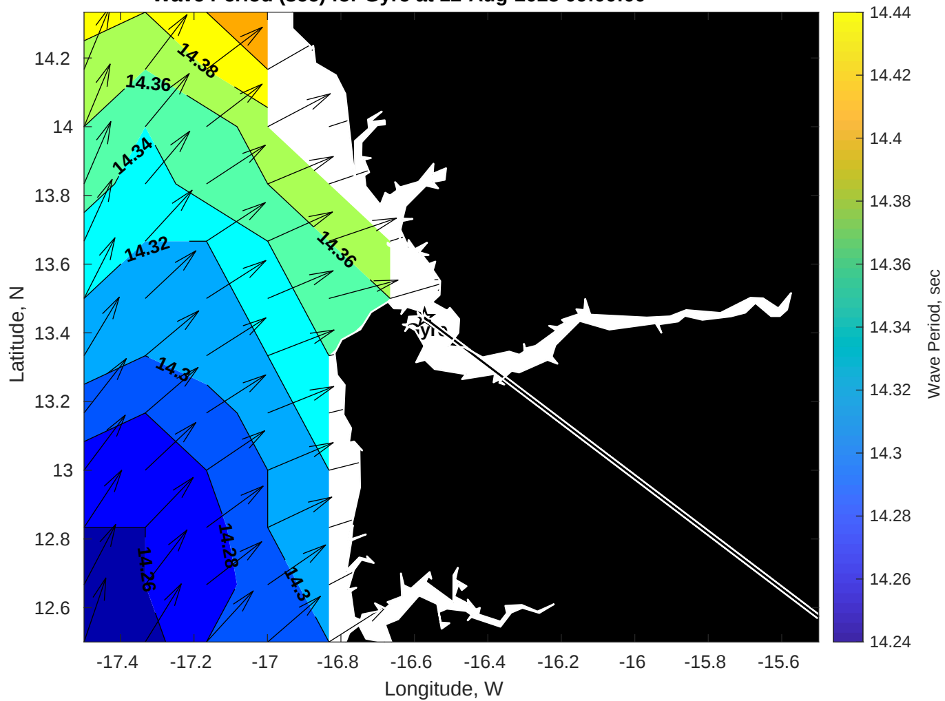
Wave Period (sec) for Gyre at 12-Aug-2025 09:00:00
