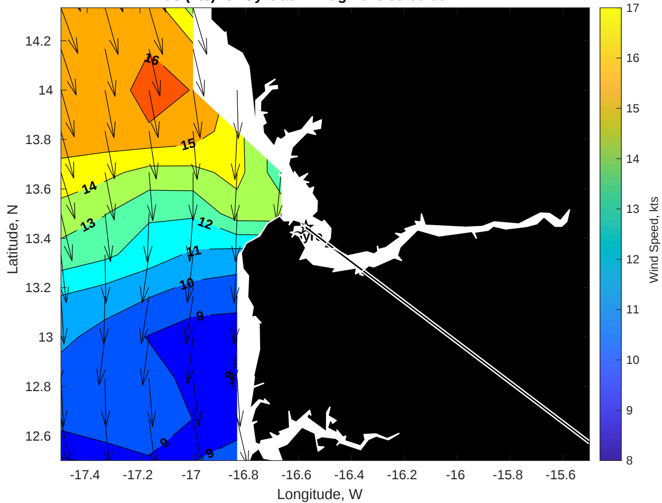
Winds (kts) for Gyre at 12-Aug-2025 09:00:00
