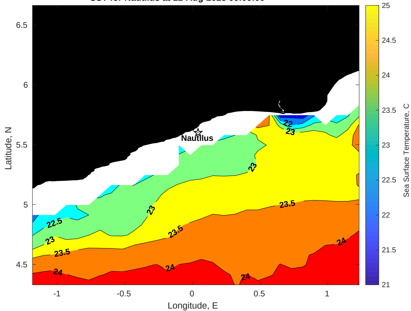
SST for Nautilus at 11-Aug-2025 00:00:00
