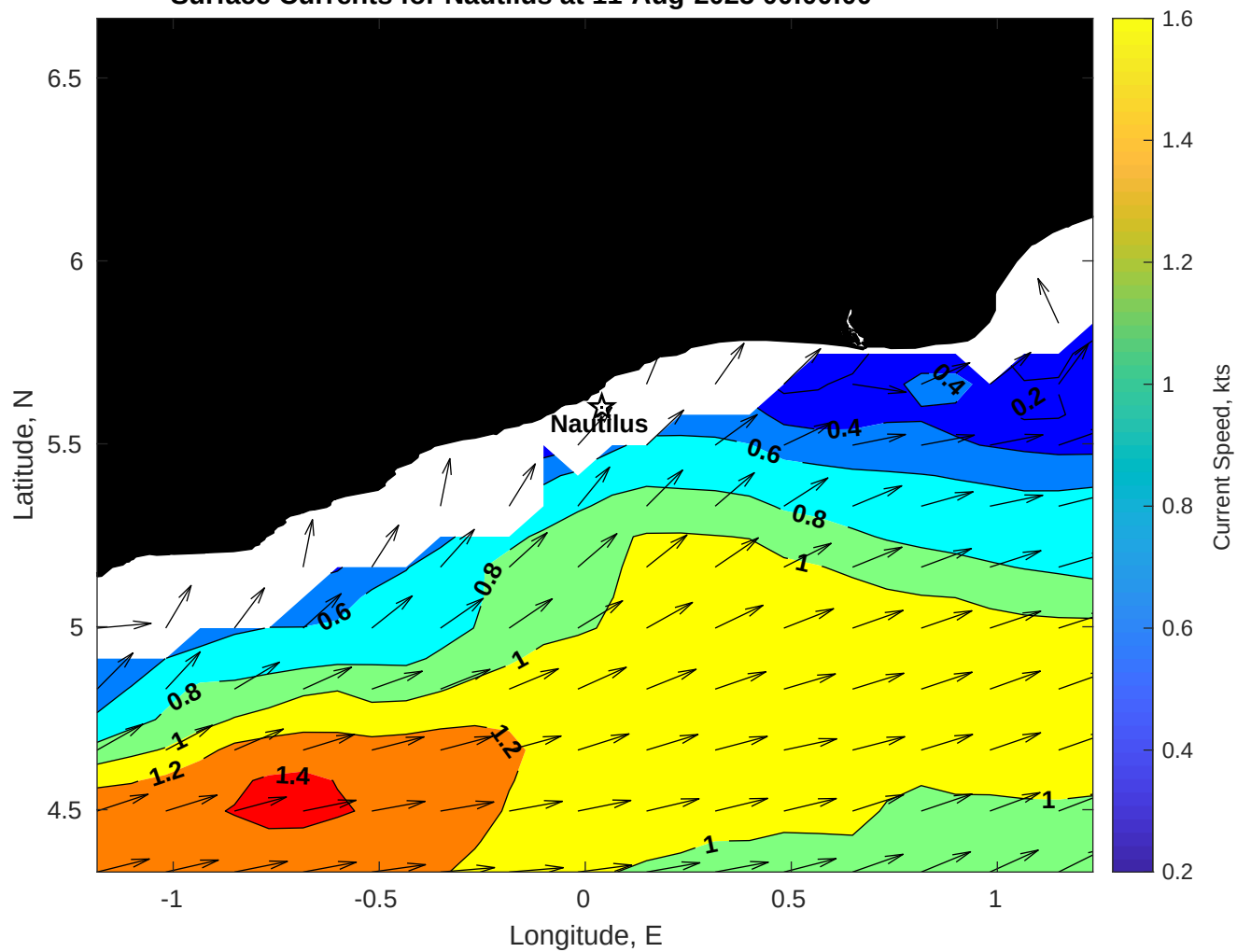
Surface Currents for Nautilus at 11-Aug-2025 00:00:00
