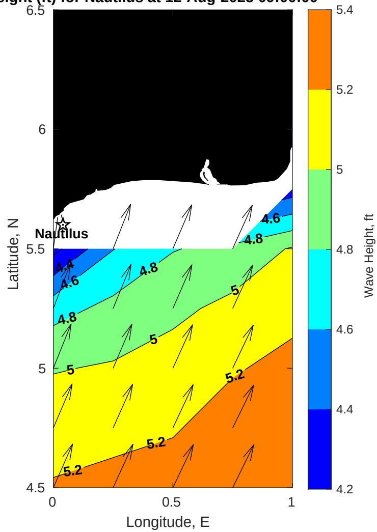
Wave Height (ft) for Nautilus at 12-Aug-2025 09:00:00
