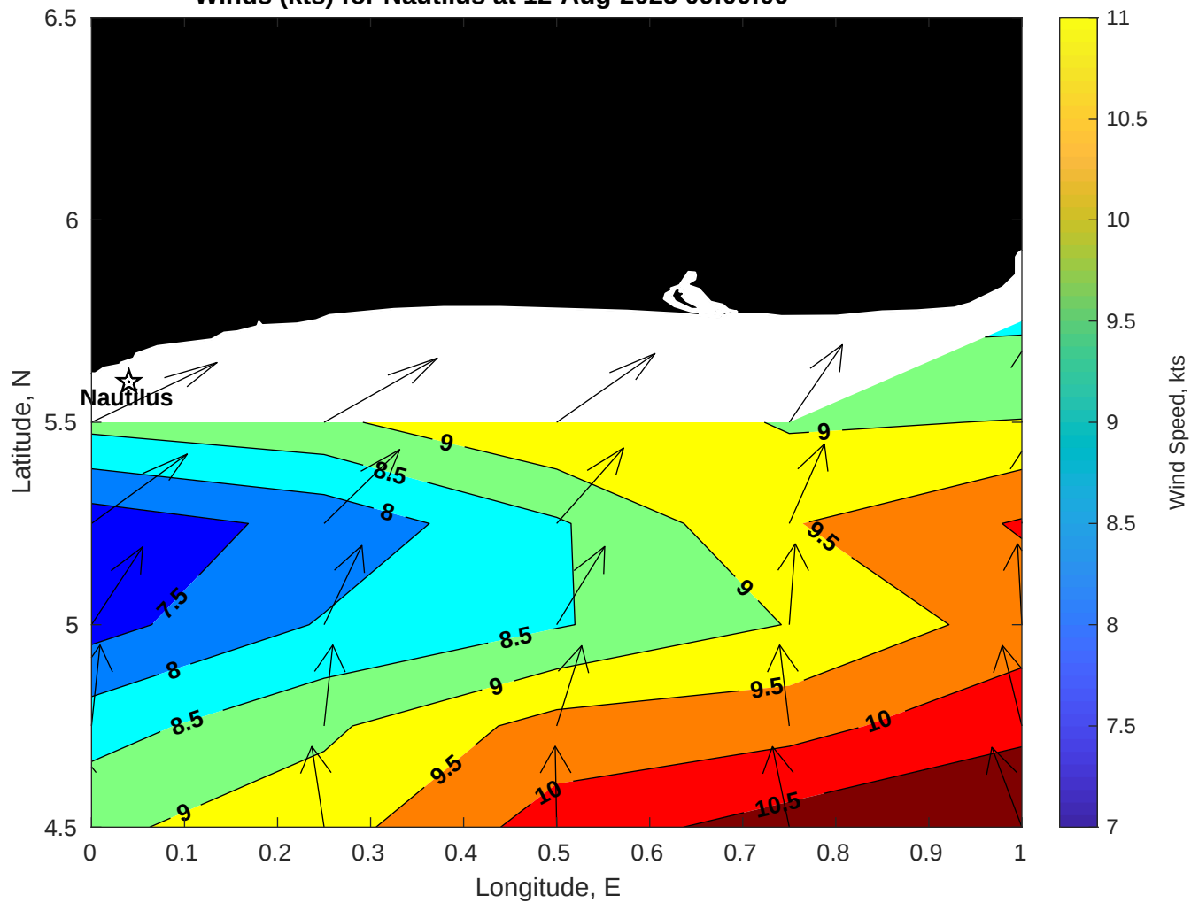
Winds (kts) for Nautilus at 12-Aug-2025 09:00:00
