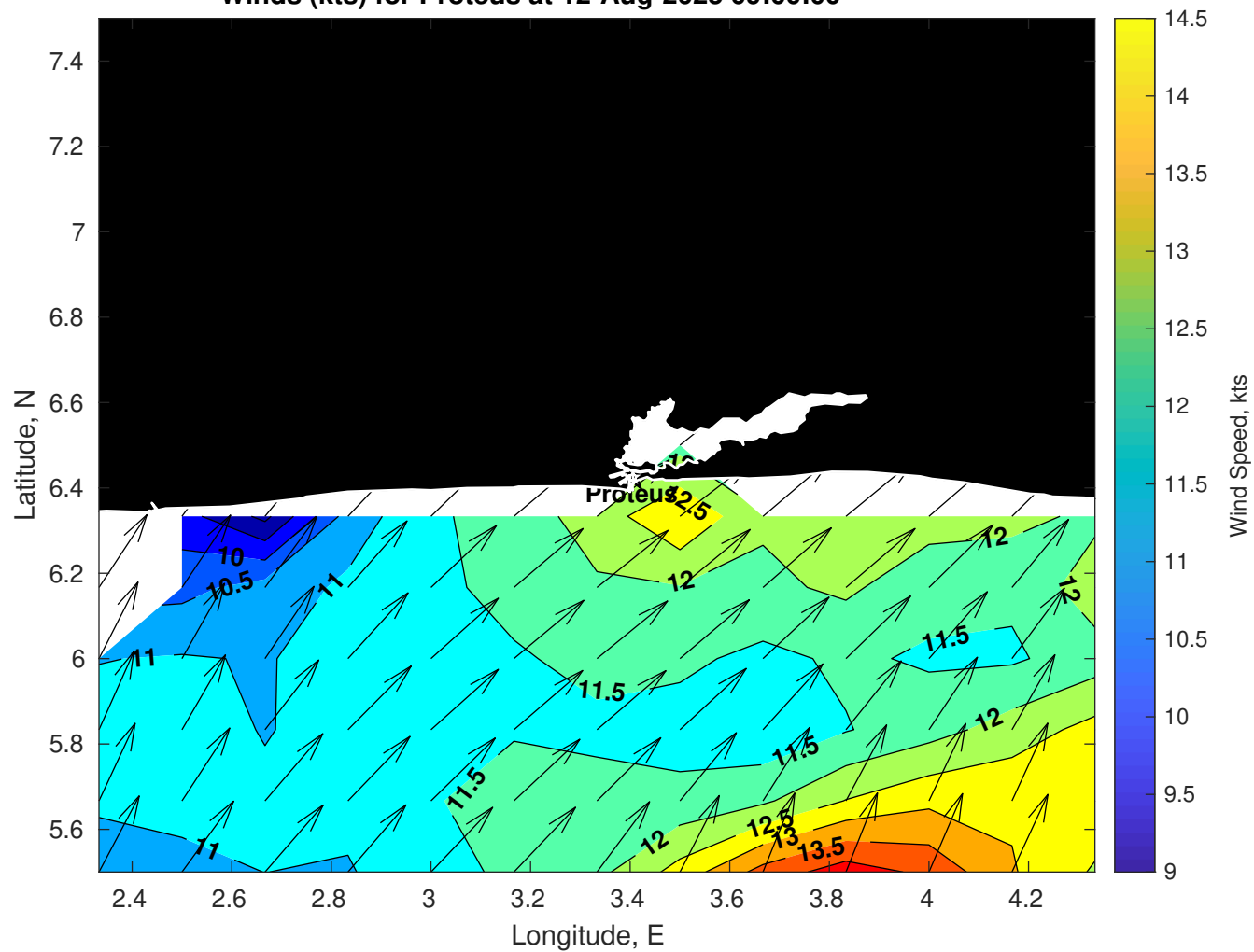
Winds (kts) for Proteus at 12-Aug-2025 09:00:00
