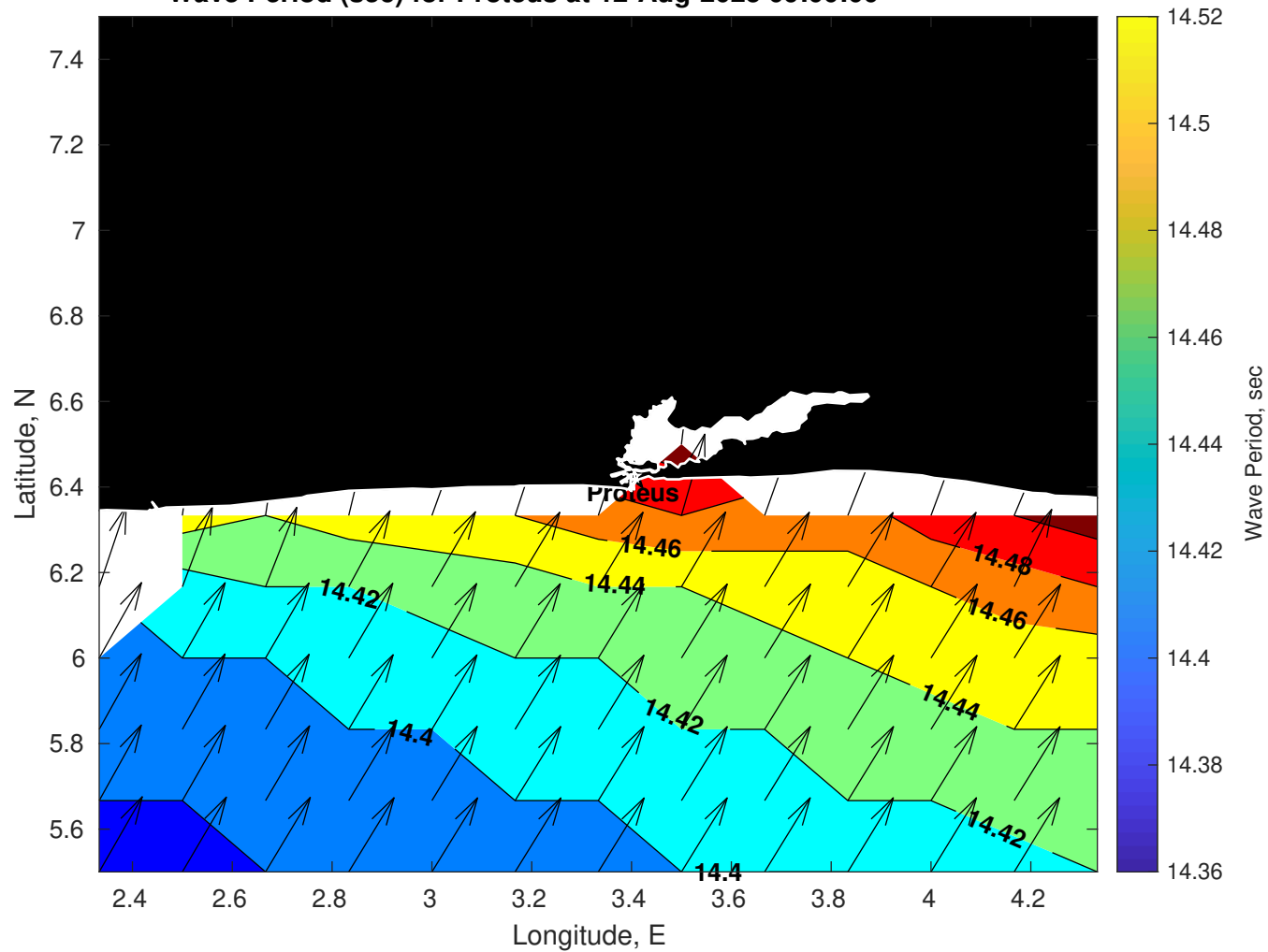
Wave Period (sec) for Proteus at 12-Aug-2025 09:00:00
