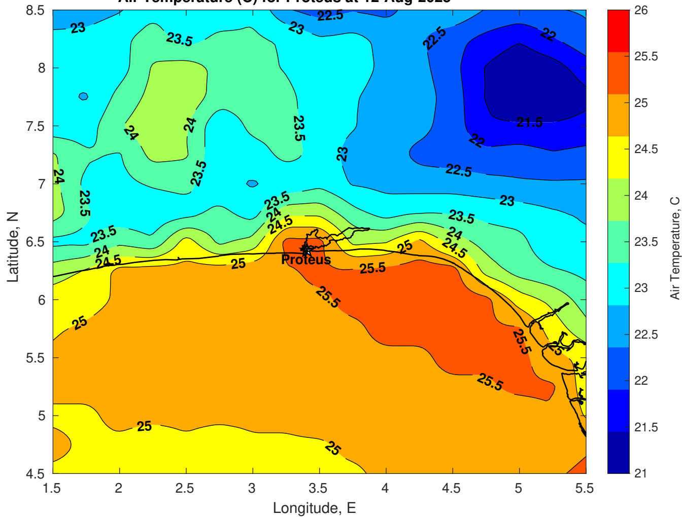
Air Temperature (C) for Proteus at 12-Aug-2025
