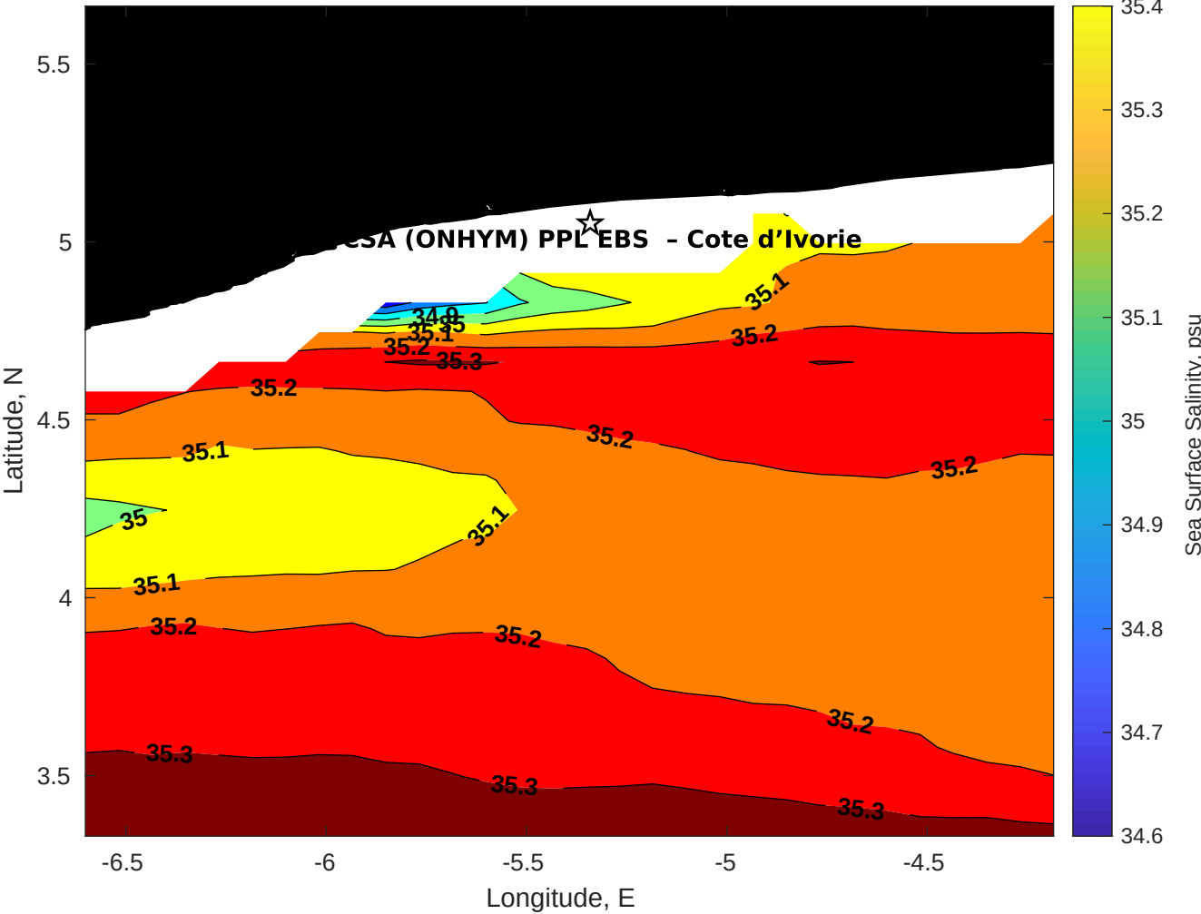
Surface Salinity for CSA (ONHYM) PPL EBS - Cote d'Ivoire at 12-Aug-2025 00:00:00
