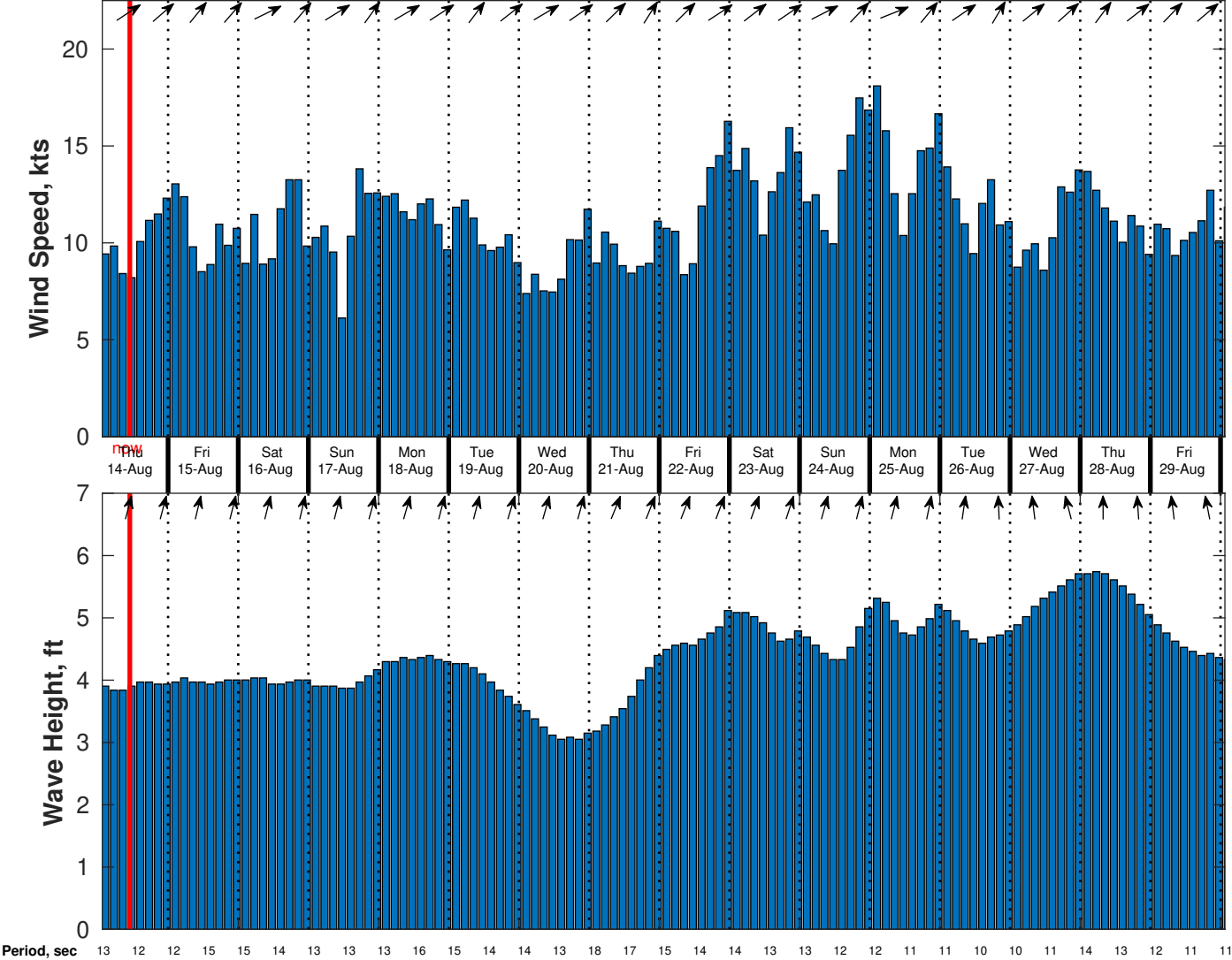
Wind & Wave Forecast for CSA (ONHYM) PPL EBS - Cote d'Ivoire from 13-Aug-2025 01:00:00 to 29-Aug-2025 01:00:00
