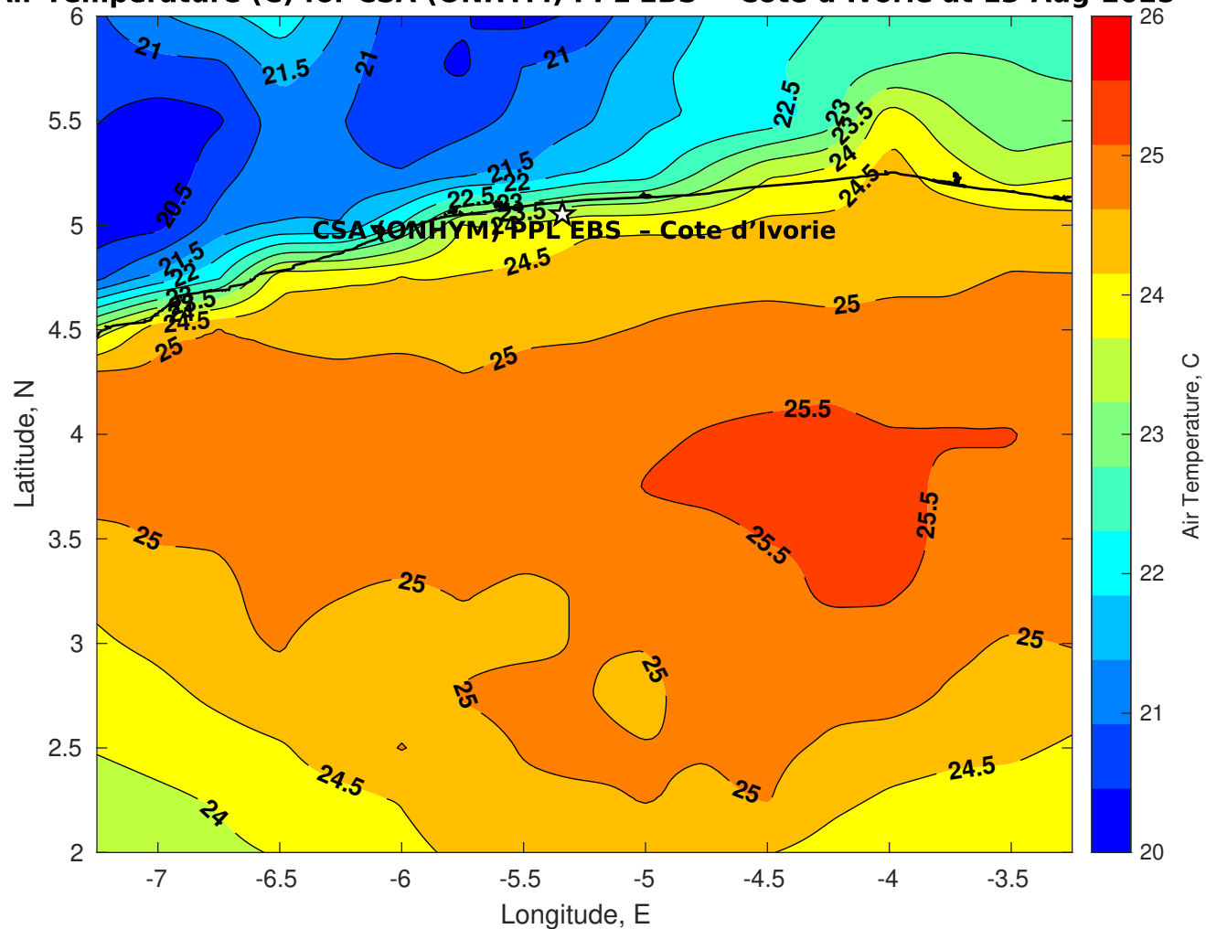
Air Temperature (C) for CSA (ONHYM) PPL EBS - Cote d'Ivoire at 13-Aug-2025
