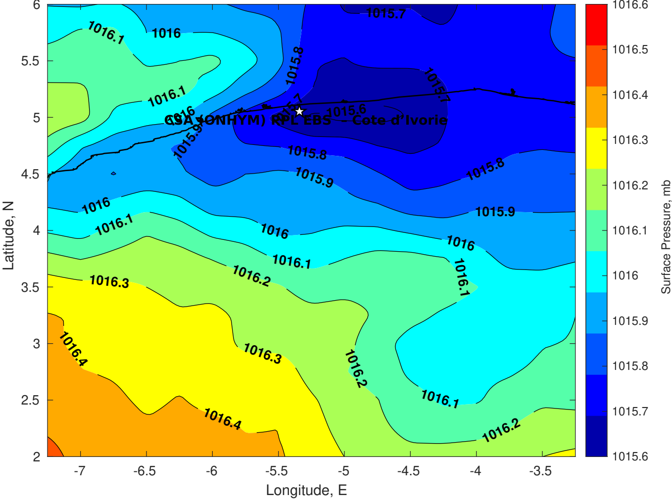
Surface Pressure (mb) for CSA (ONHYM) PPL EBS - Cote d'Ivoire at 14-Aug-2025 00:00:00
