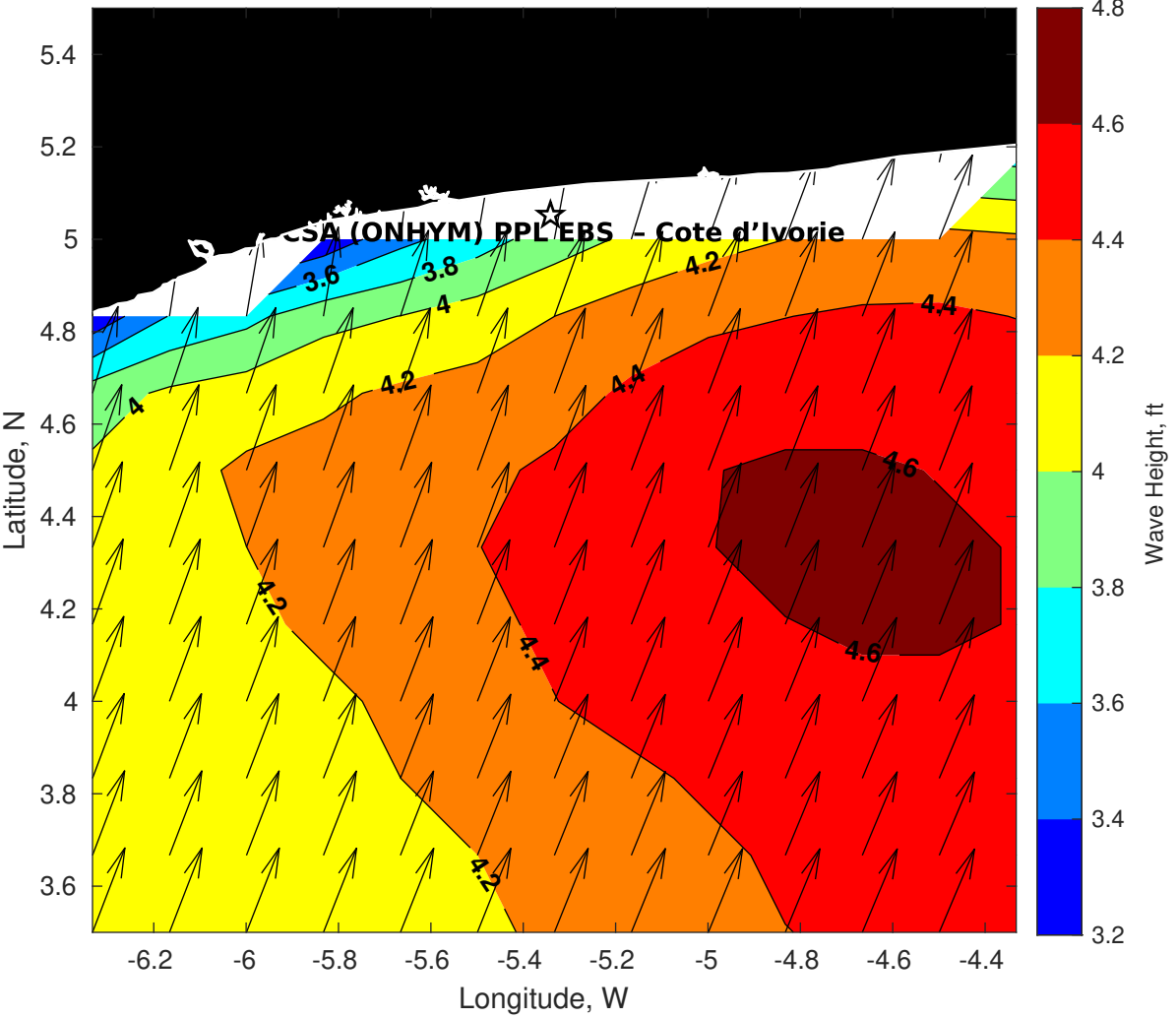
Wave Height (ft) for CSA (ONHYM) PPL EBS - Cote d'Ivoire at 13-Aug-2025 09:00:00
