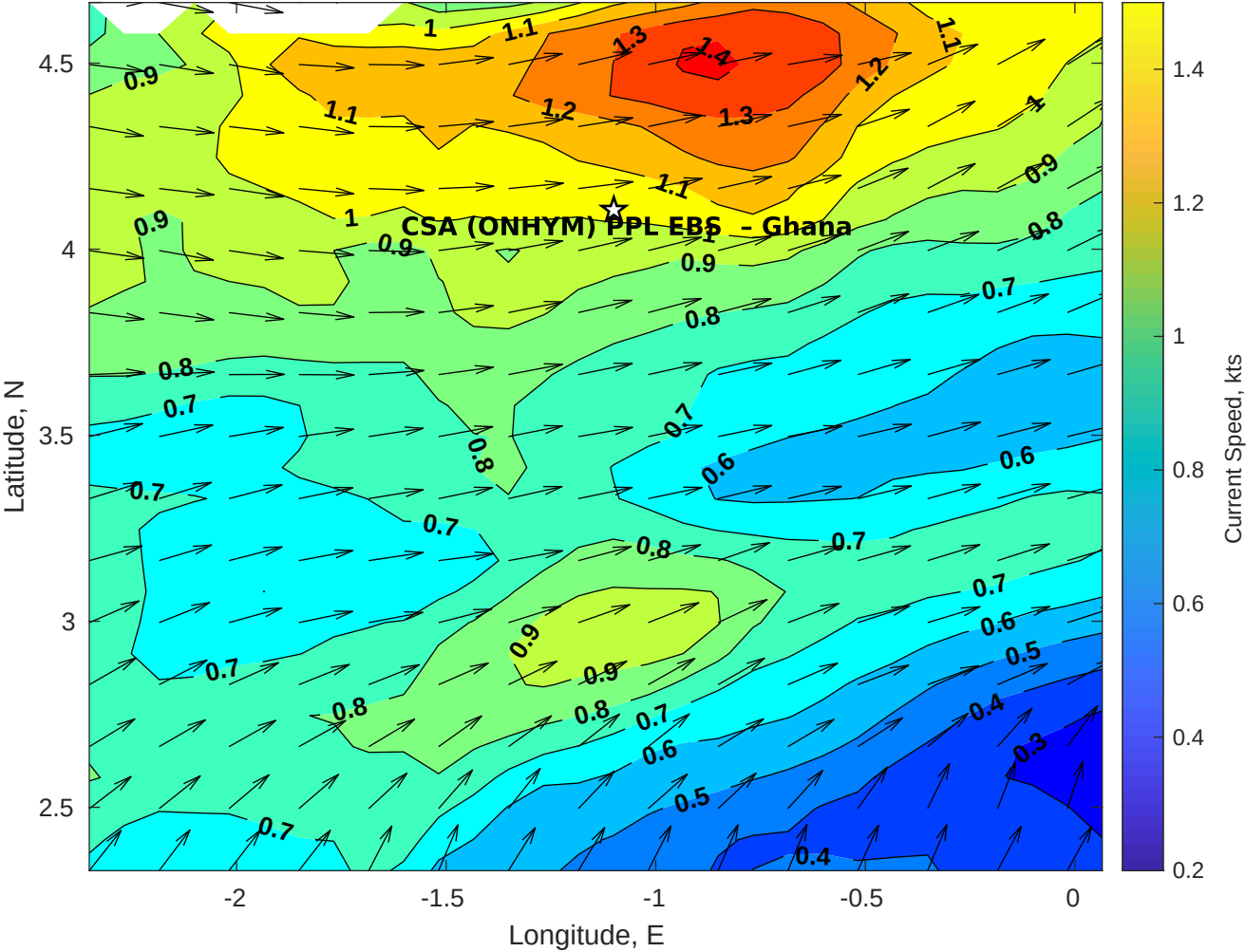
Surface Currents for CSA (ONHYM) PPL EBS - Ghana at 12-Aug-2025 00:00:00
