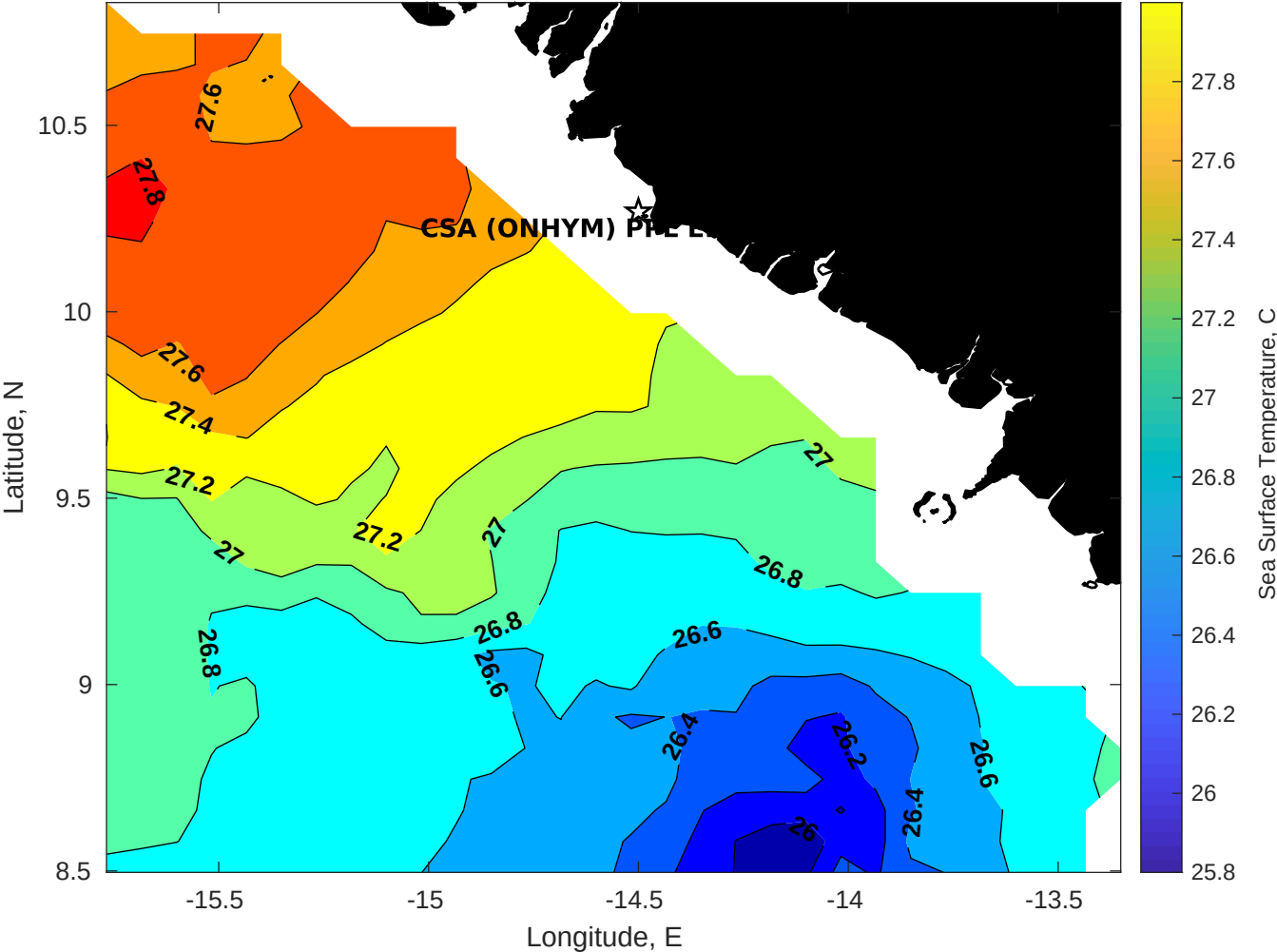
SST for CSA (ONHYM) PPL EBS - Guinea at 12-Aug-2025 00:00:00
