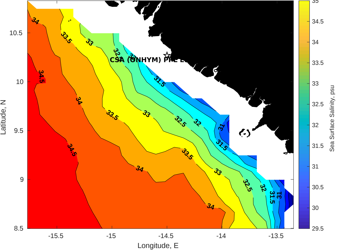
Surface Salinity for CSA (ONHYM) PPL EBS - Guinea at 12-Aug-2025 00:00:00
