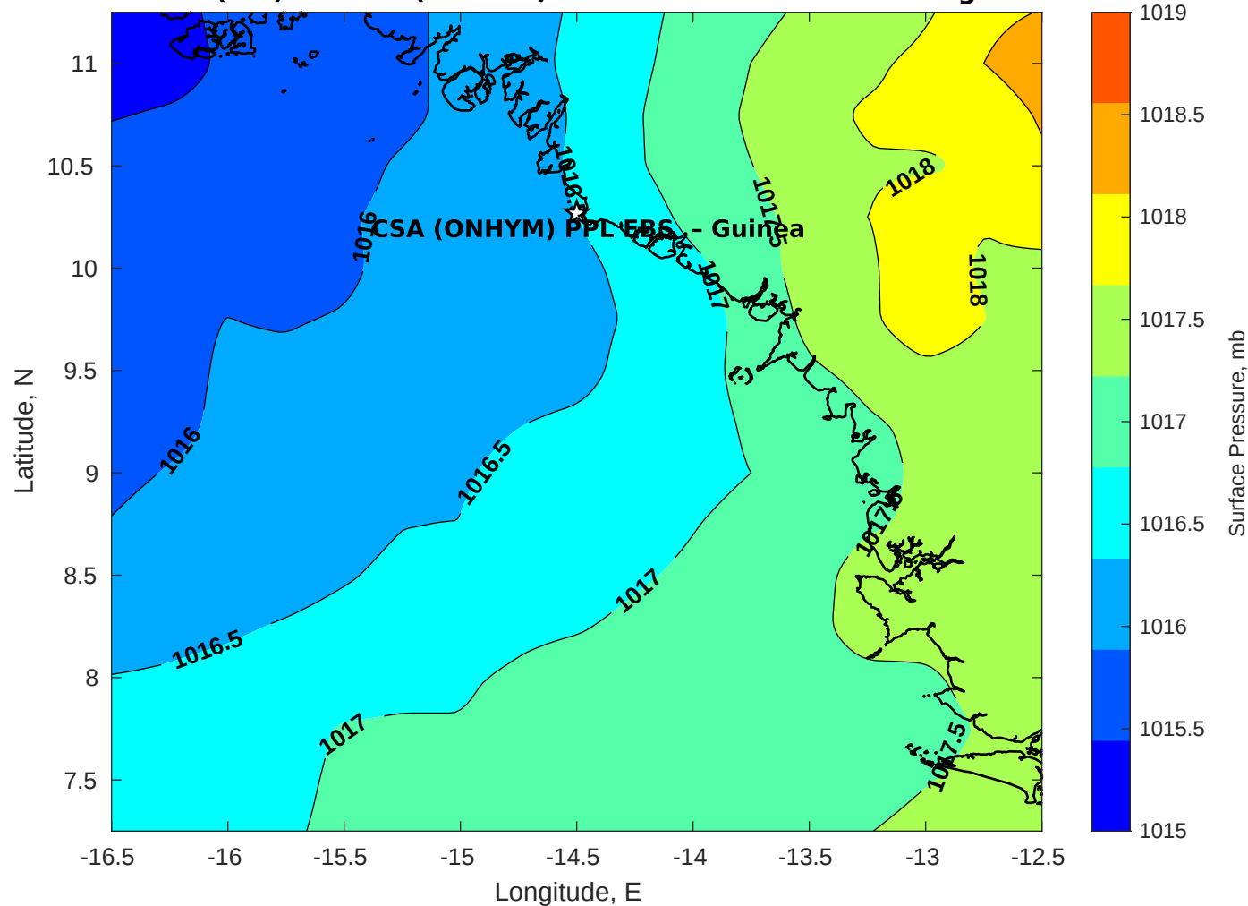
Surface Pressure (mb) for CSA (ONHYM) PPL EBS - Guinea at 15-Aug-2025 00:00:00
