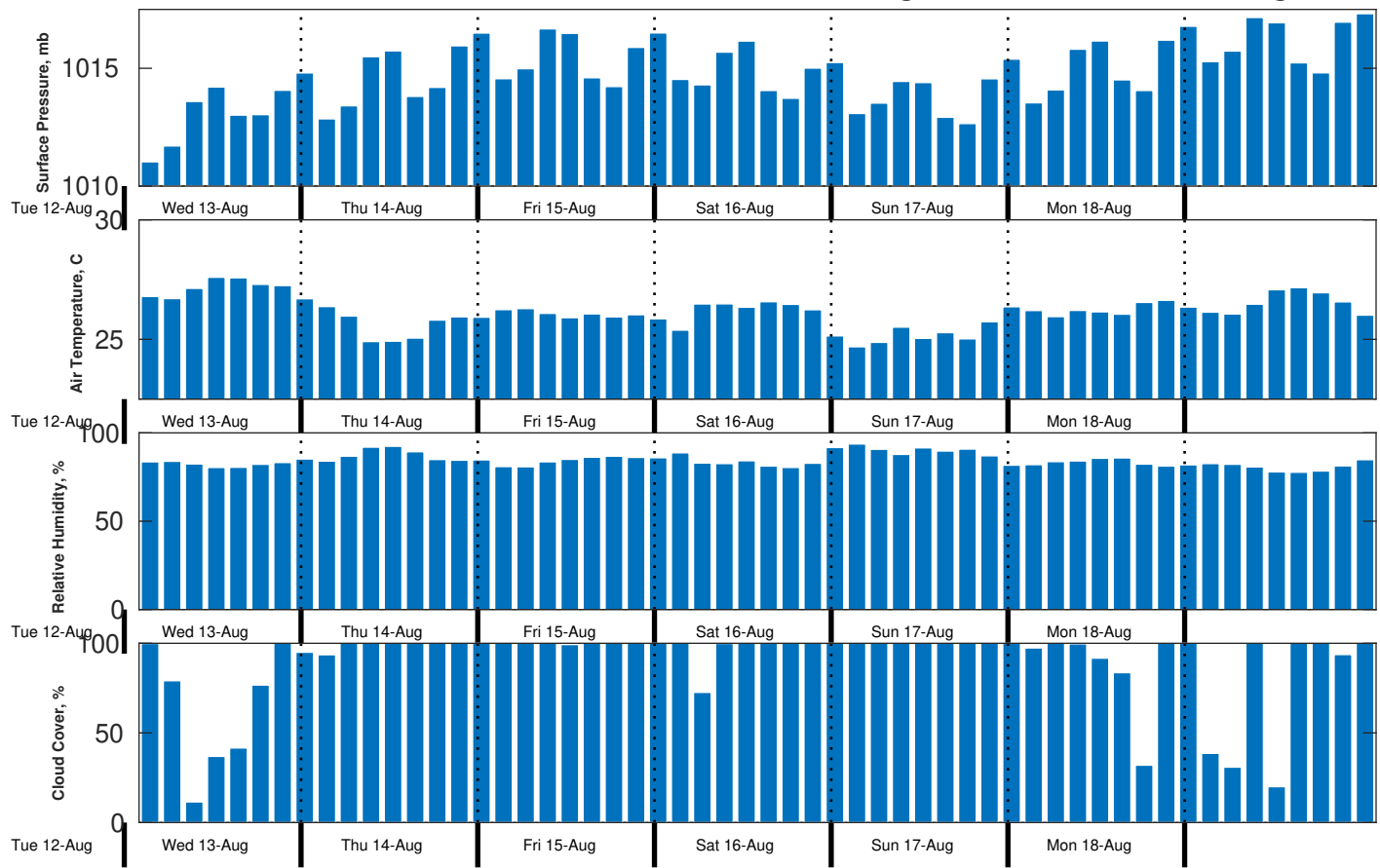
Met Forecast for CSA (ONHYM) PPL EBS - Guinea from 13-Aug-2025 00:00:00 to 20-Aug-2025 00:00:00
