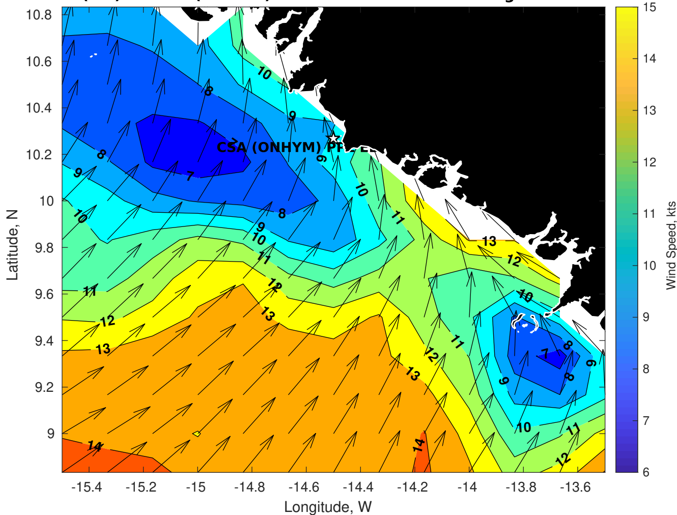
Winds (kts) for CSA (ONHYM) PPL EBS - Guinea at 13-Aug-2025 09:00:00
