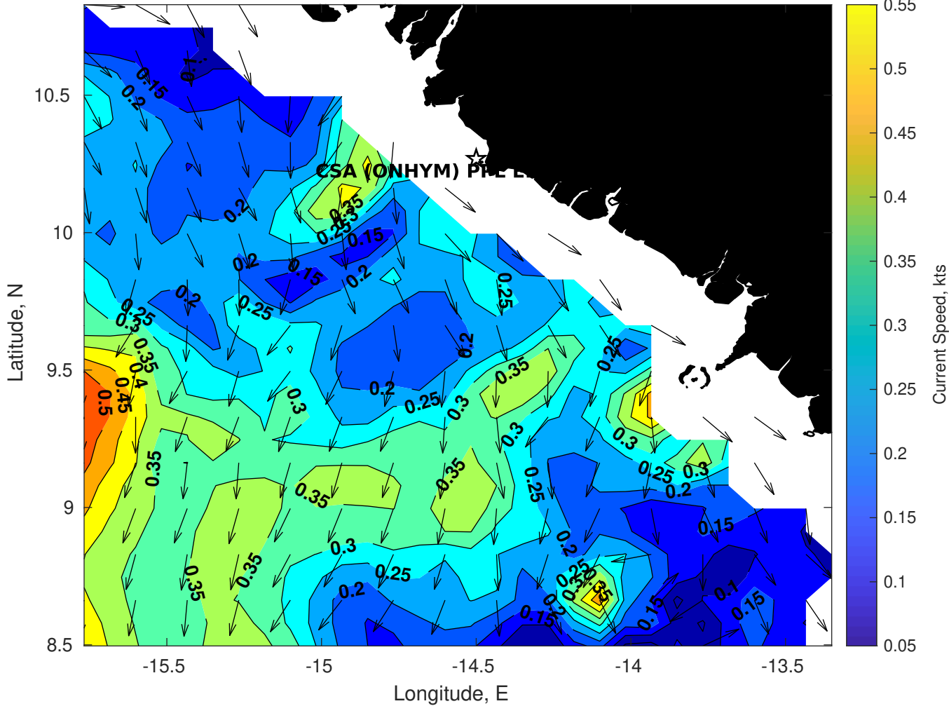
Surface Currents for CSA (ONHYM) PPL EBS - Guinea at 12-Aug-2025 00:00:00
