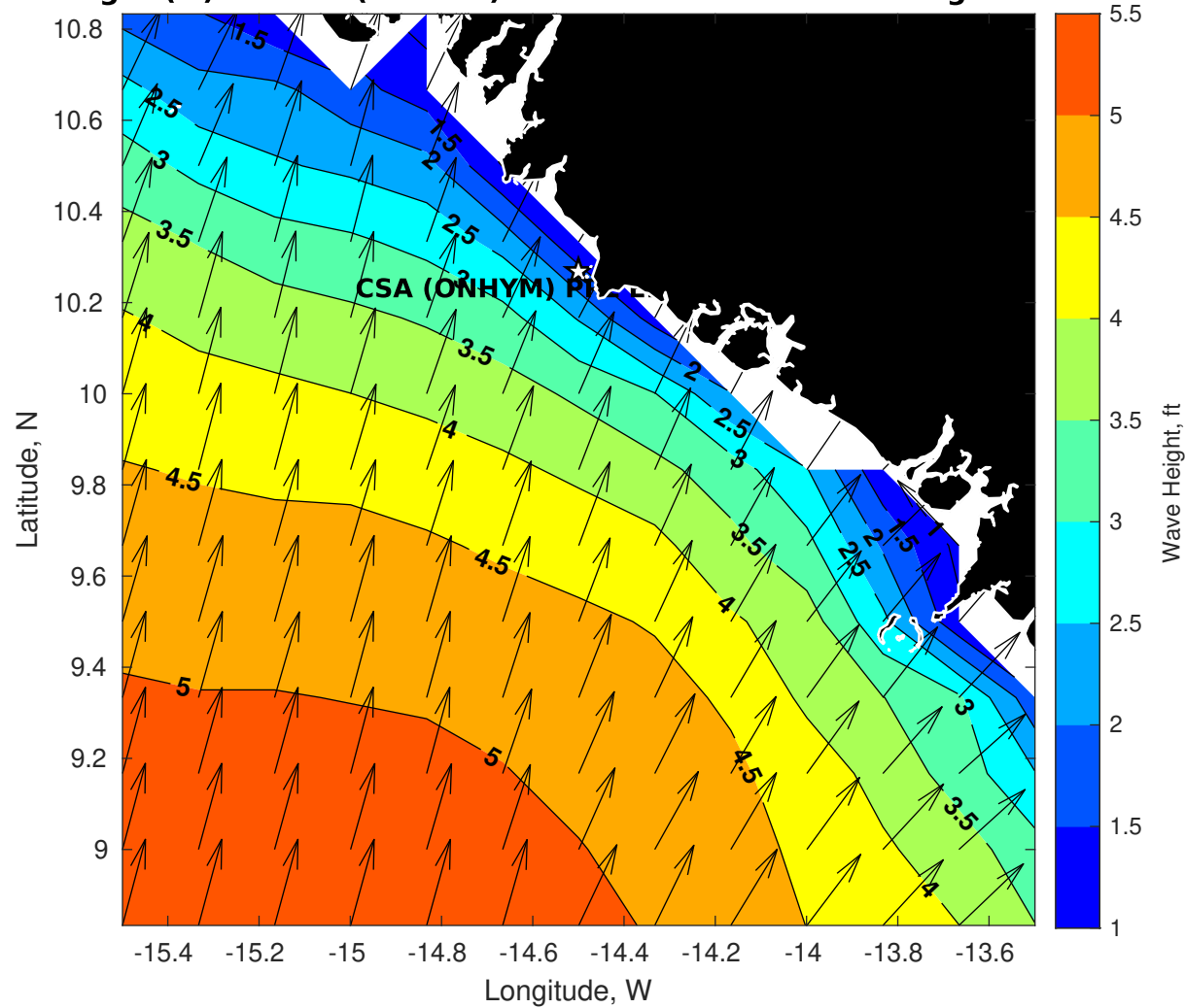
Wave Height (ft) for CSA (ONHYM) PPL EBS - Guinea at 13-Aug-2025 09:00:00
