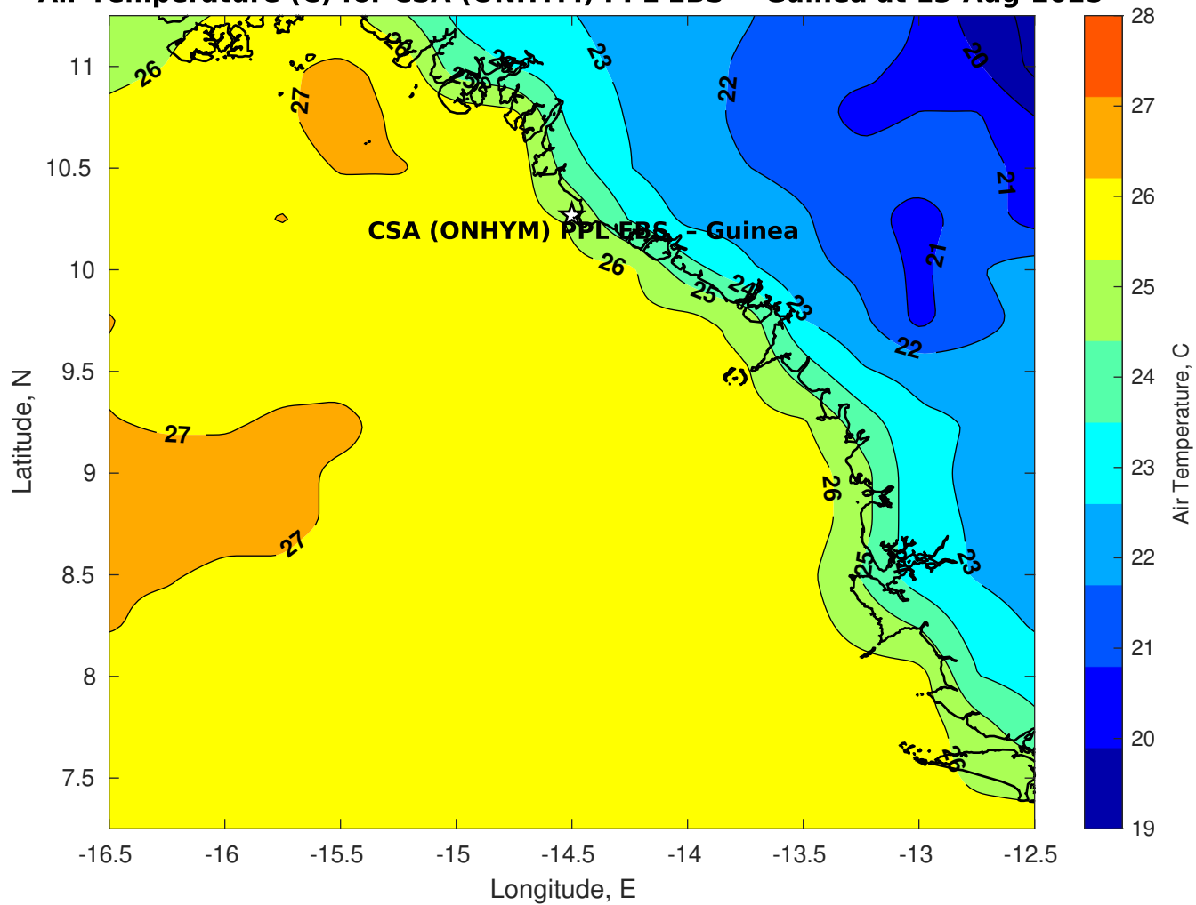
Air Temperature (C) for CSA (ONHYM) PPL EBS - Guinea at 13-Aug-2025
