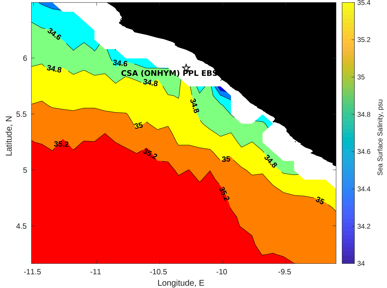
Surface Salinity for CSA (ONHYM) PPL EBS - Liberia at 12-Aug-2025 00:00:00
