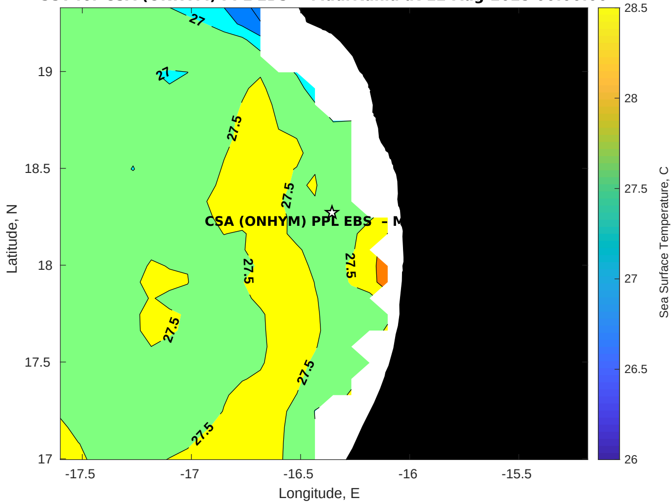
SST for CSA (ONHYM) PPL EBS - Mauritania at 12-Aug-2025 00:00:00
