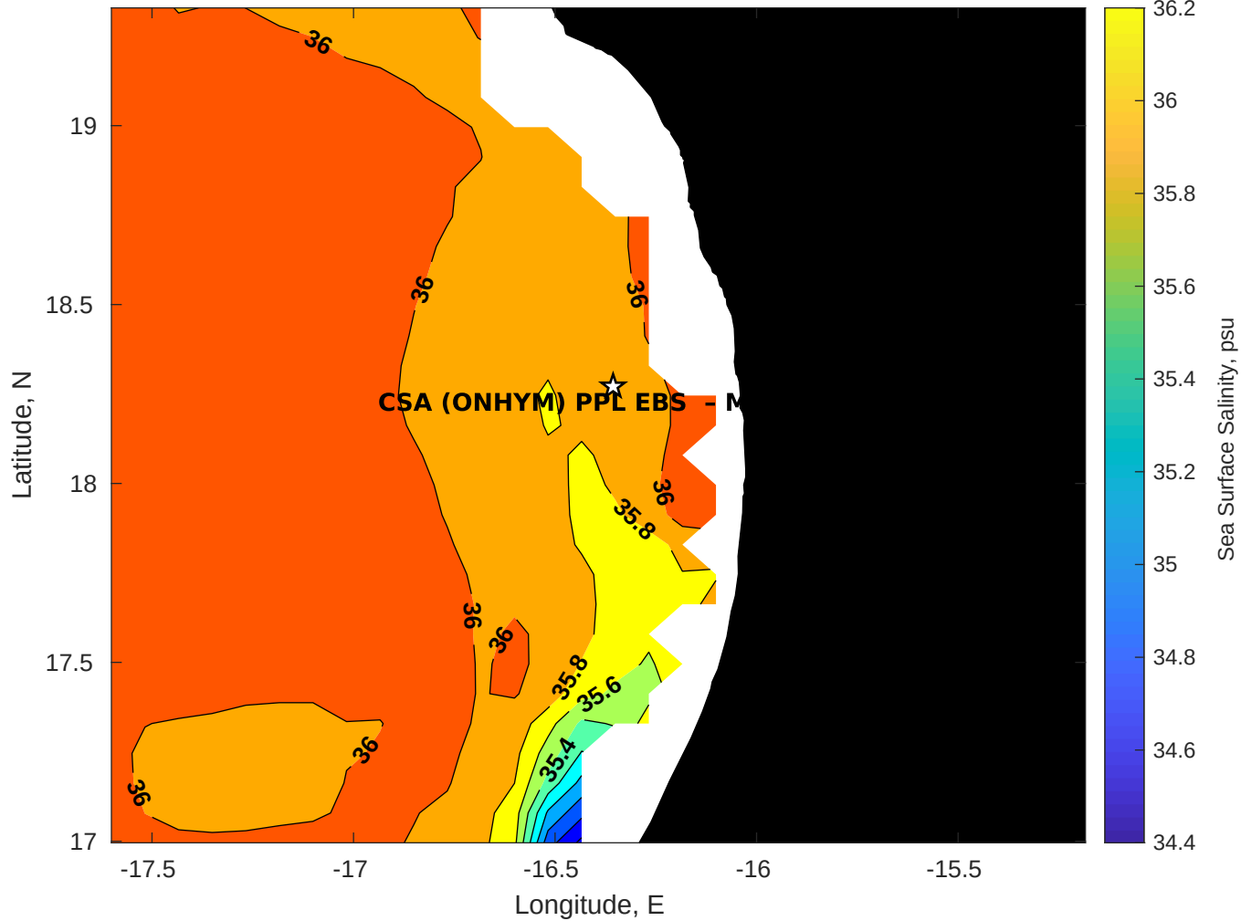
Surface Salinity for CSA (ONHYM) PPL EBS - Mauritania at 12-Aug-2025 00:00:00
