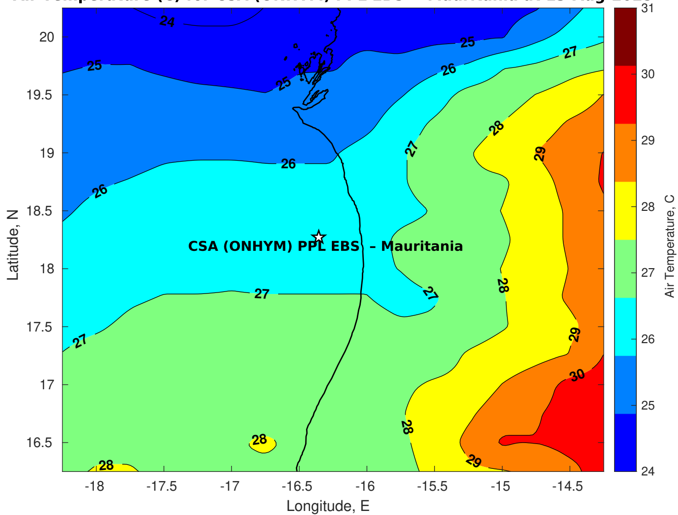
Air Temperature (C) for CSA (ONHYM) PPL EBS - Mauritania at 13-Aug-2025
