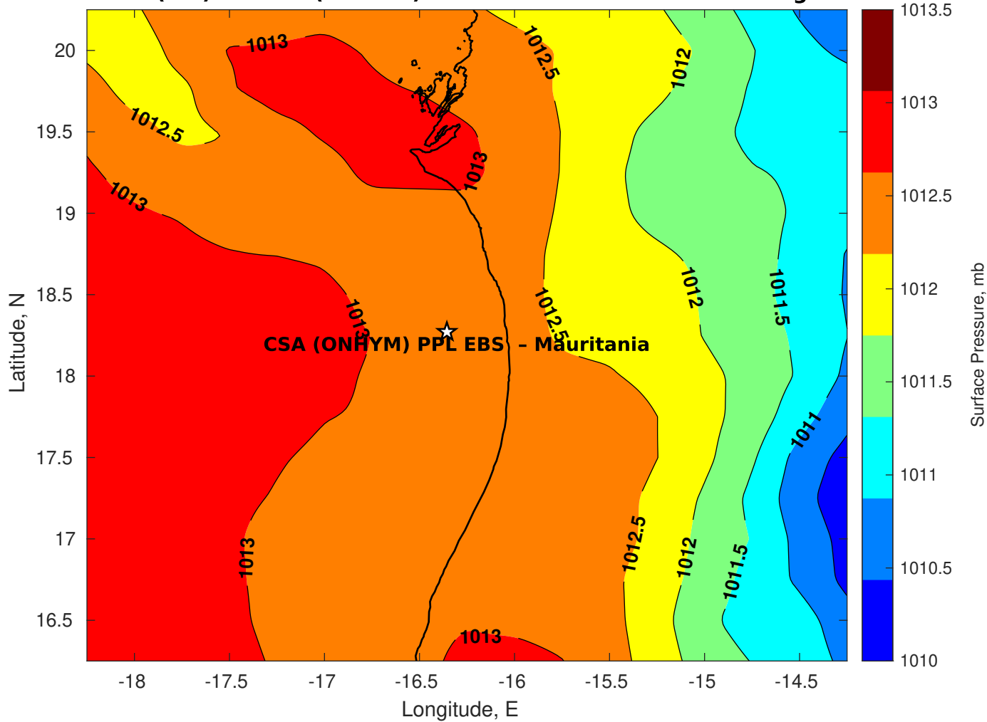
Surface Pressure (mb) for CSA (ONHYM) PPL EBS - Mauritania at 14-Aug-2025 00:00:00
