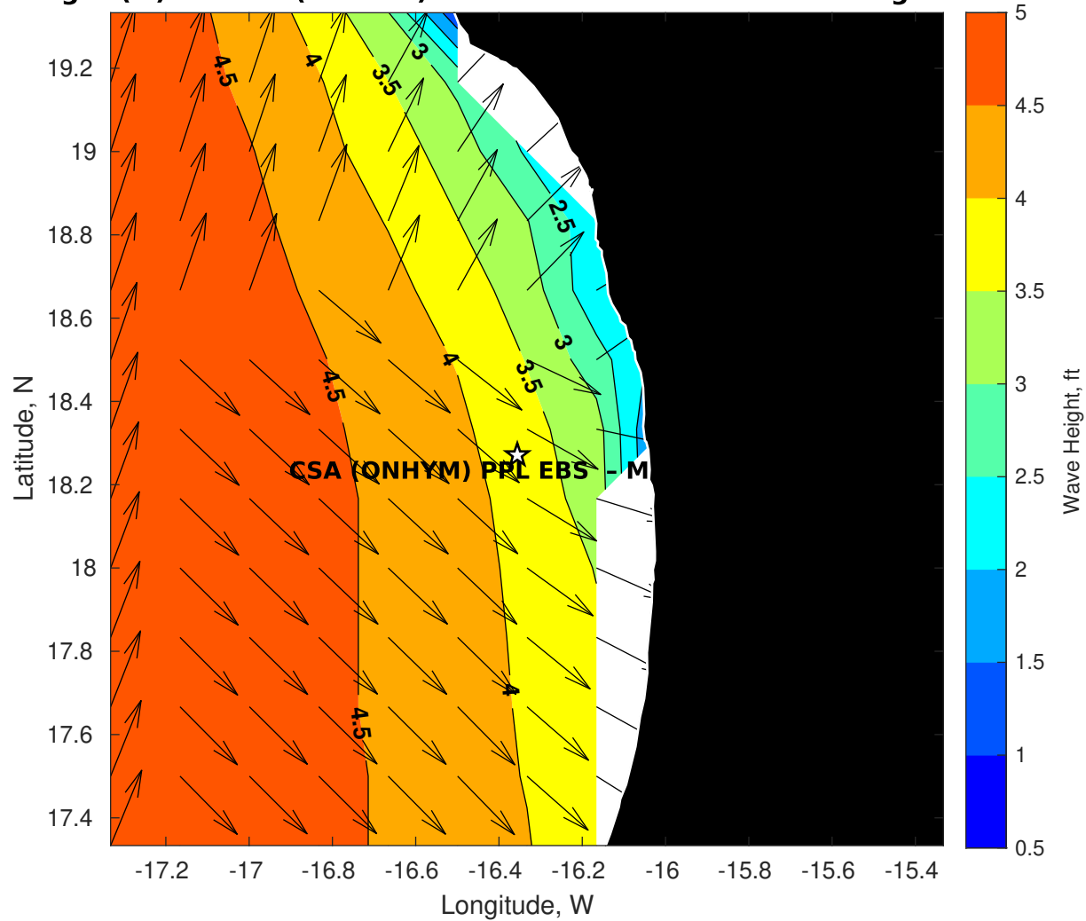
Wave Height (ft) for CSA (ONHYM) PPL EBS - Mauritania at 13-Aug-2025 09:00:00
