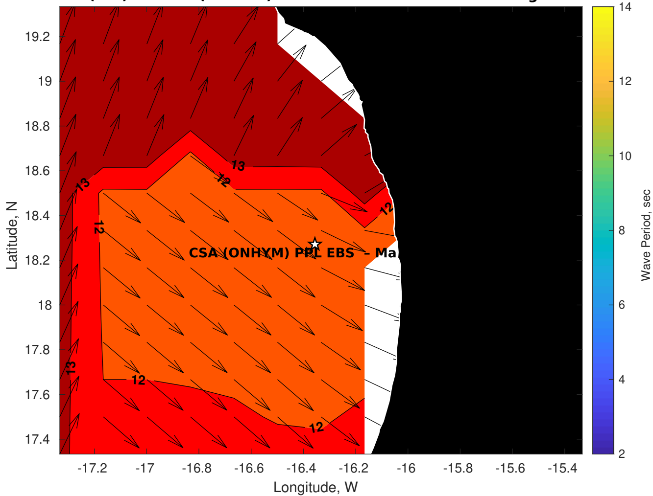
Wave Period (sec) for CSA (ONHYM) PPL EBS - Mauritania at 13-Aug-2025 09:00:00
