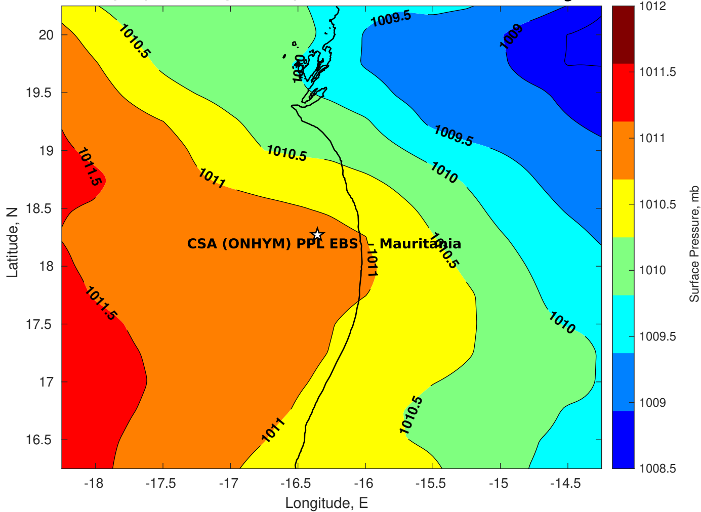
Surface Pressure (mb) for CSA (ONHYM) PPL EBS - Mauritania at 13-Aug-2025 00:00:00
