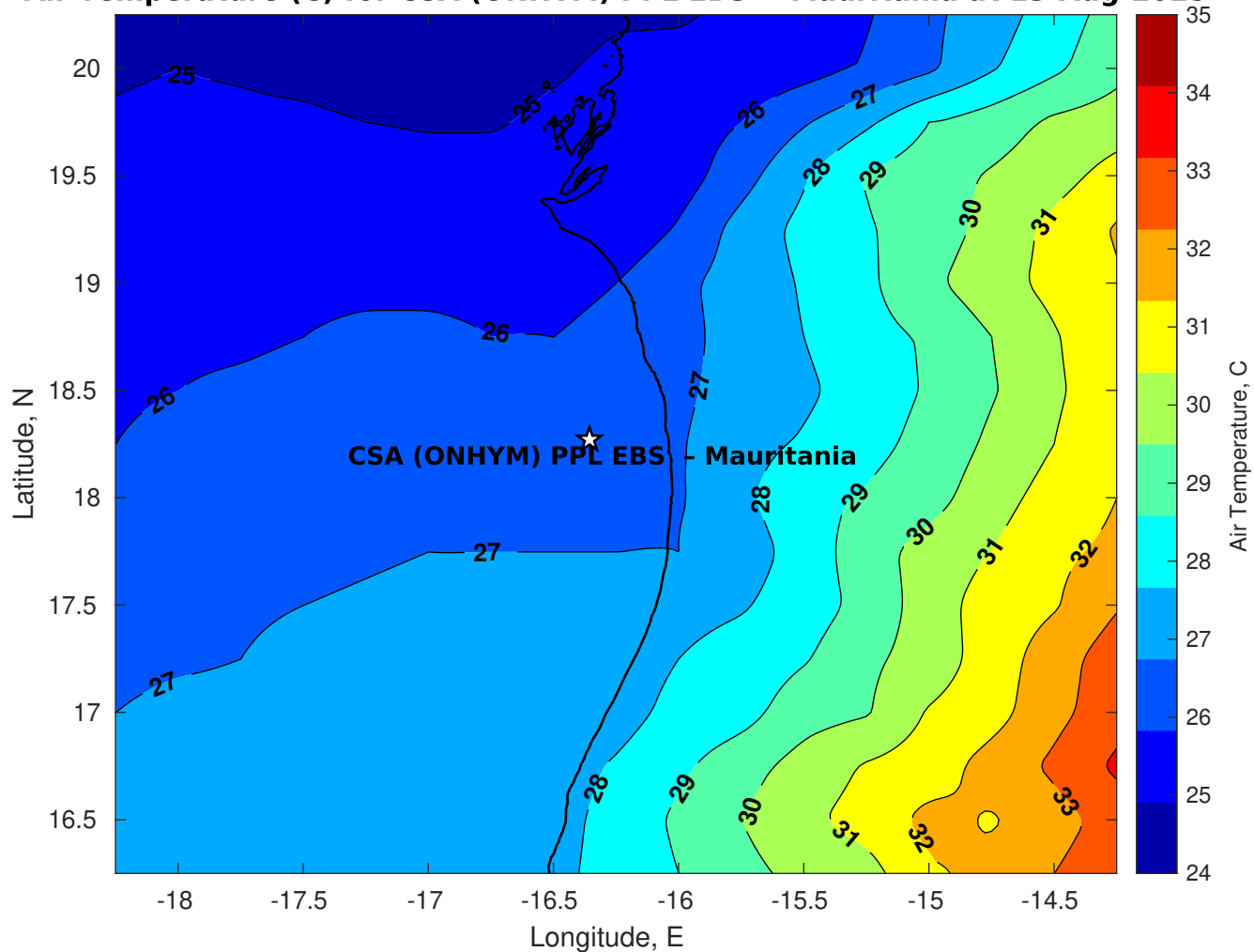
Air Temperature (C) for CSA (ONHYM) PPL EBS - Mauritania at 13-Aug-2025
