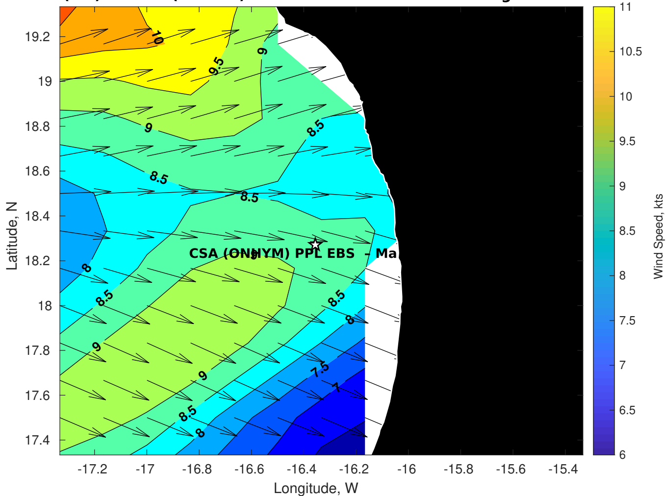
Winds (kts) for CSA (ONHYM) PPL EBS - Mauritania at 13-Aug-2025 09:00:00
