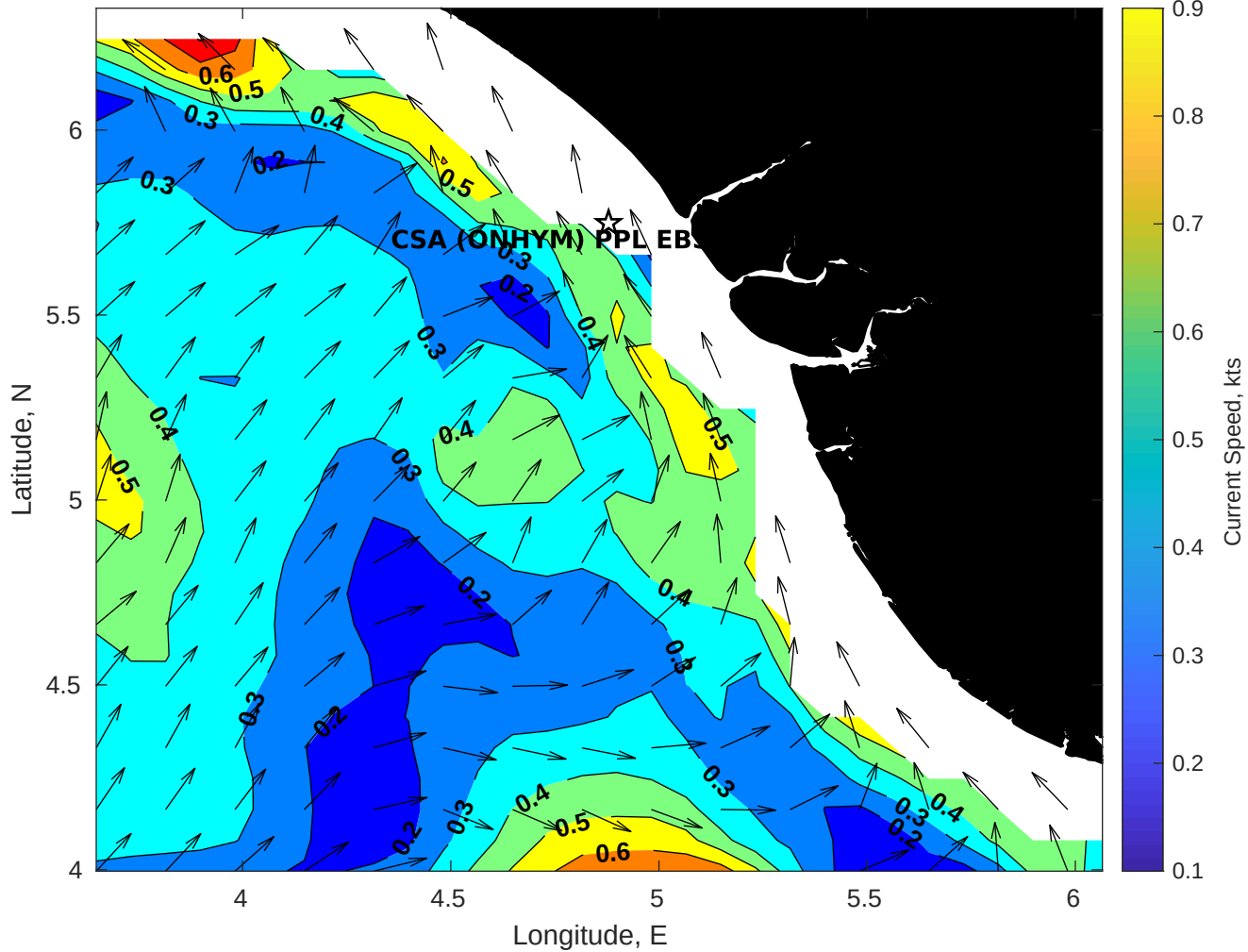
Surface Currents for CSA (ONHYM) PPL EBS - Nigeria at 12-Aug-2025 00:00:00
