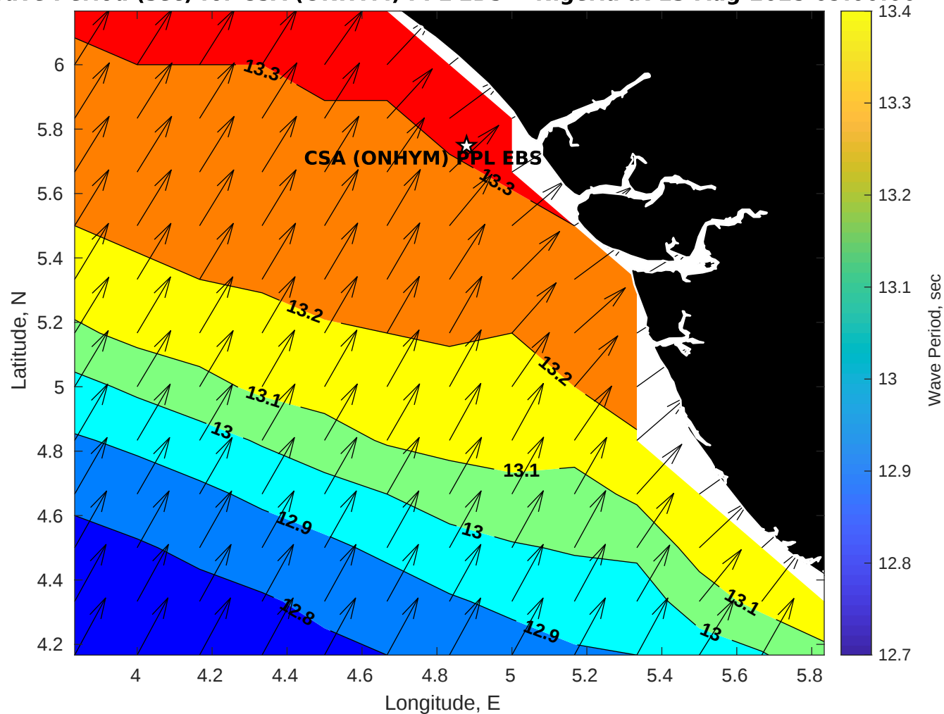
Wave Period (sec) for CSA (ONHYM) PPL EBS - Nigeria at 13-Aug-2025 09:00:00
