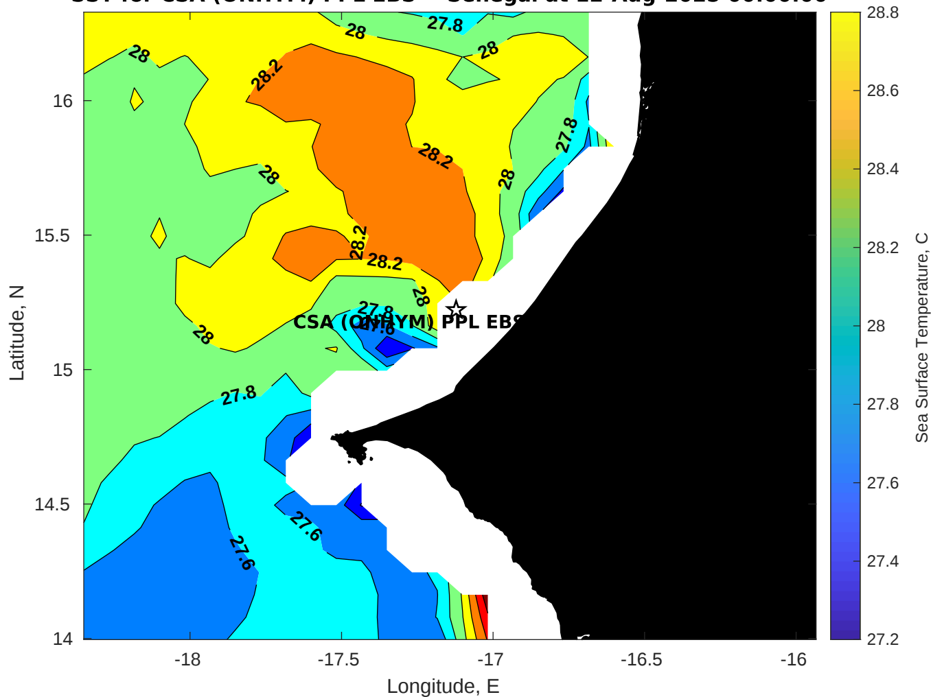
SST for CSA (ONHYM) PPL EBS - Senegal at 12-Aug-2025 00:00:00
