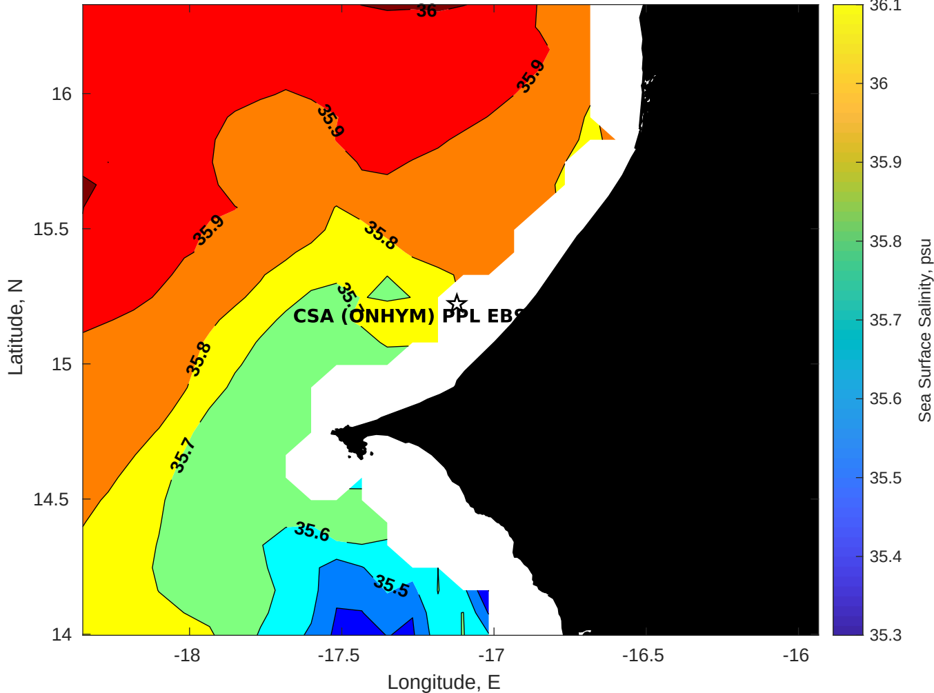
Surface Salinity for CSA (ONHYM) PPL EBS - Senegal at 12-Aug-2025 00:00:00
