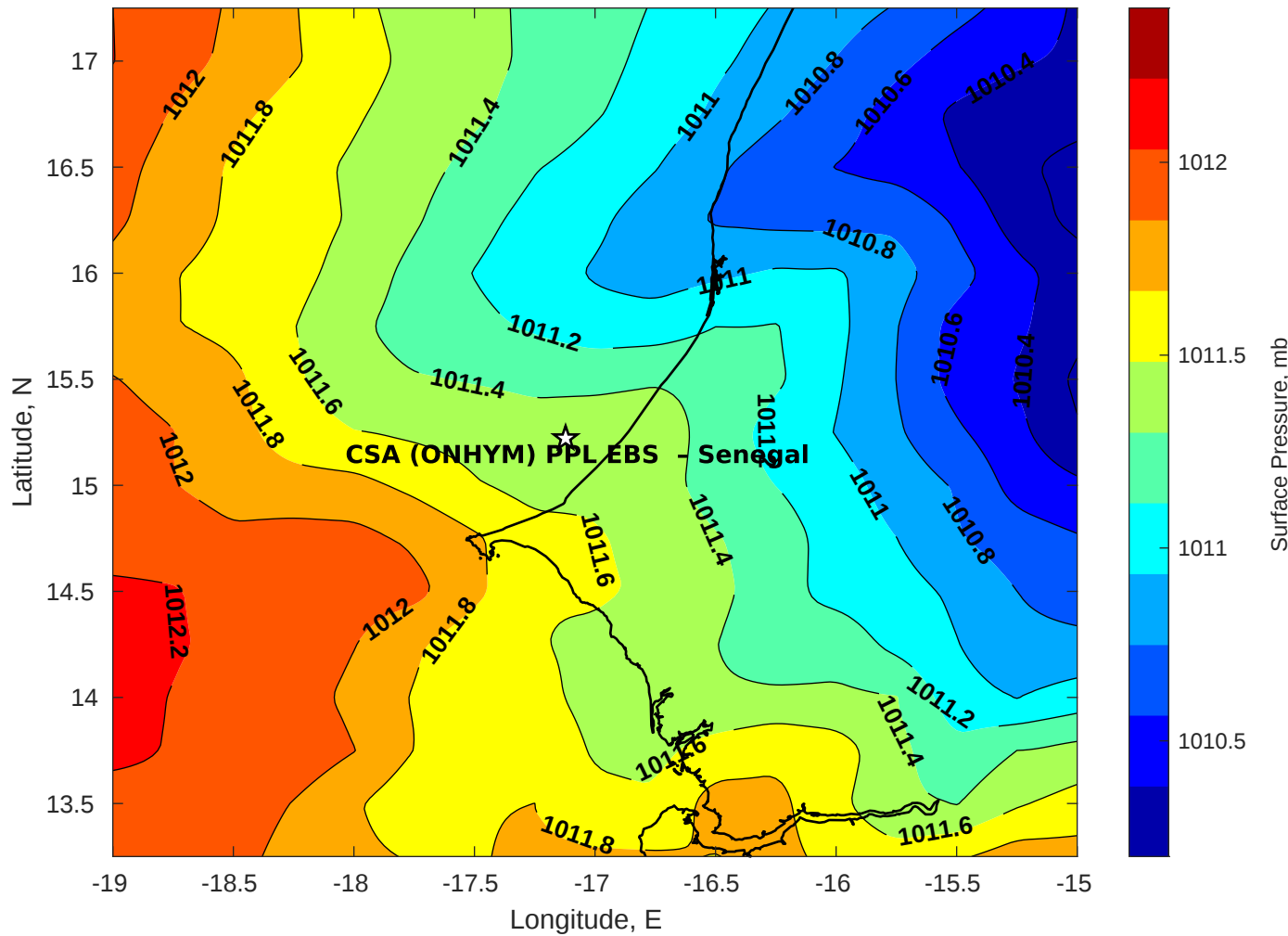
Surface Pressure (mb) for CSA (ONHYM) PPL EBS - Senegal at 13-Aug-2025 00:00:00
