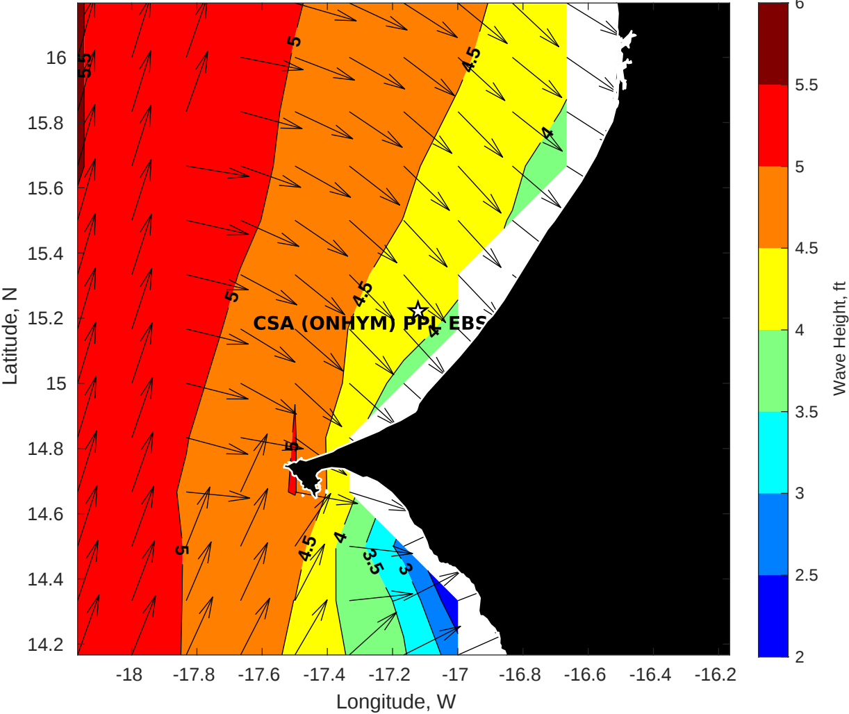
Wave Height (ft) for CSA (ONHYM) PPL EBS - Senegal at 13-Aug-2025 09:00:00
