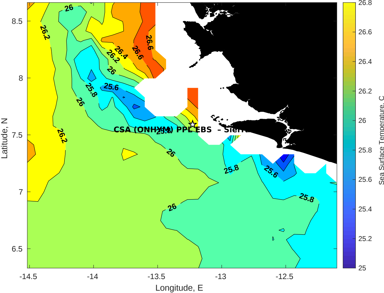
SST for CSA (ONHYM) PPL EBS - Sierra Leone at 12-Aug-2025 00:00:00
