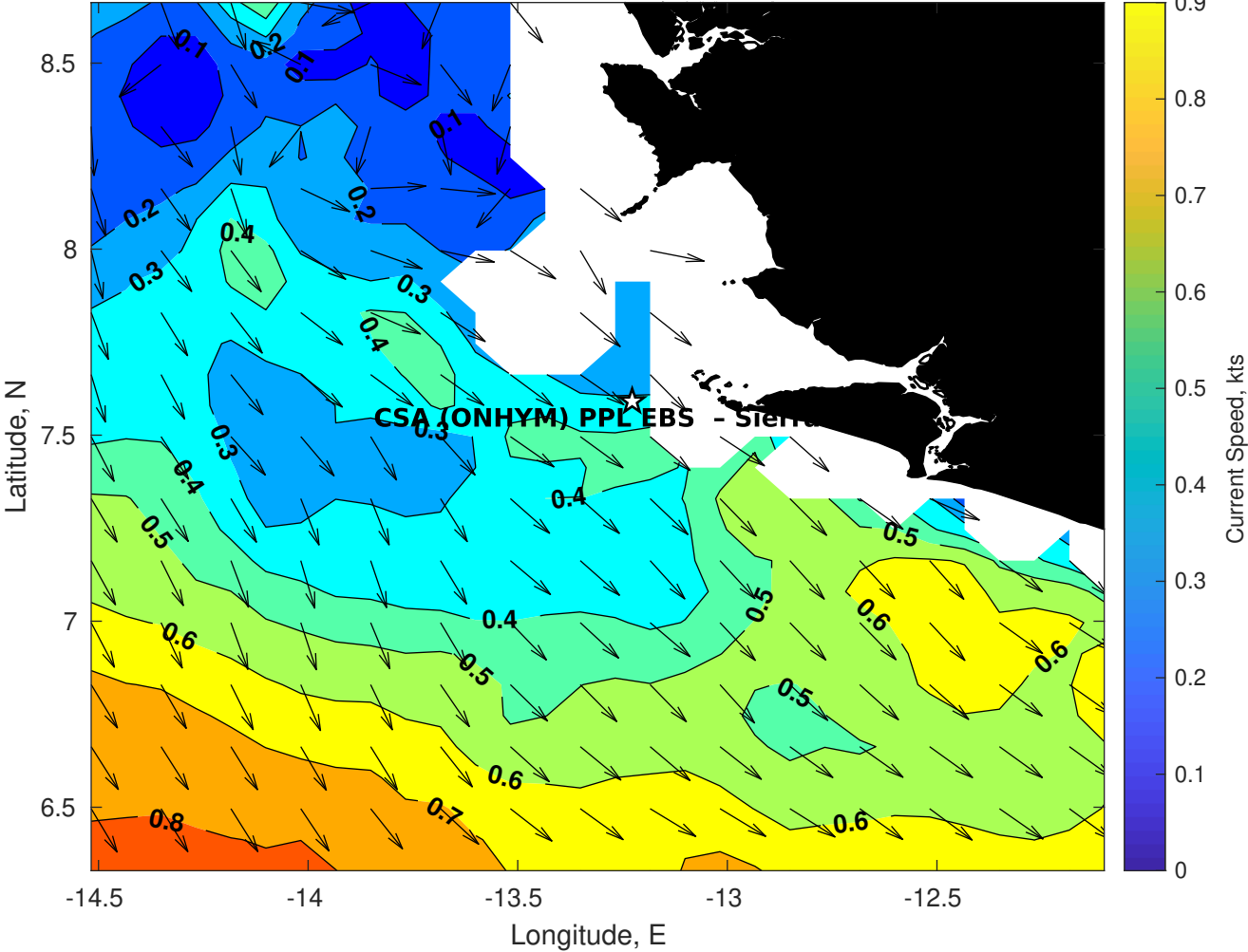
Surface Currents for CSA (ONHYM) PPL EBS - Sierra Leone at 12-Aug-2025 00:00:00
