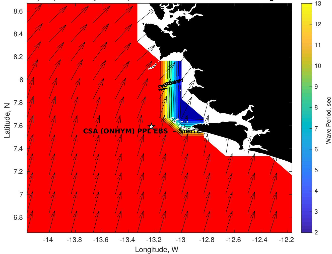
Wave Period (sec) for CSA (ONHYM) PPL EBS - Sierra Leone at 13-Aug-2025 09:00:00
