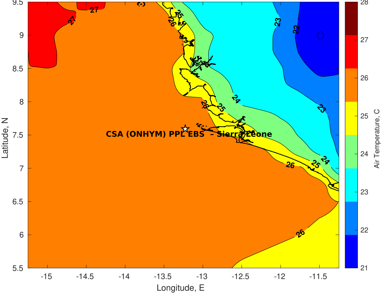
Air Temperature (C) for CSA (ONHYM) PPL EBS - Sierra Leone at 13-Aug-2025
