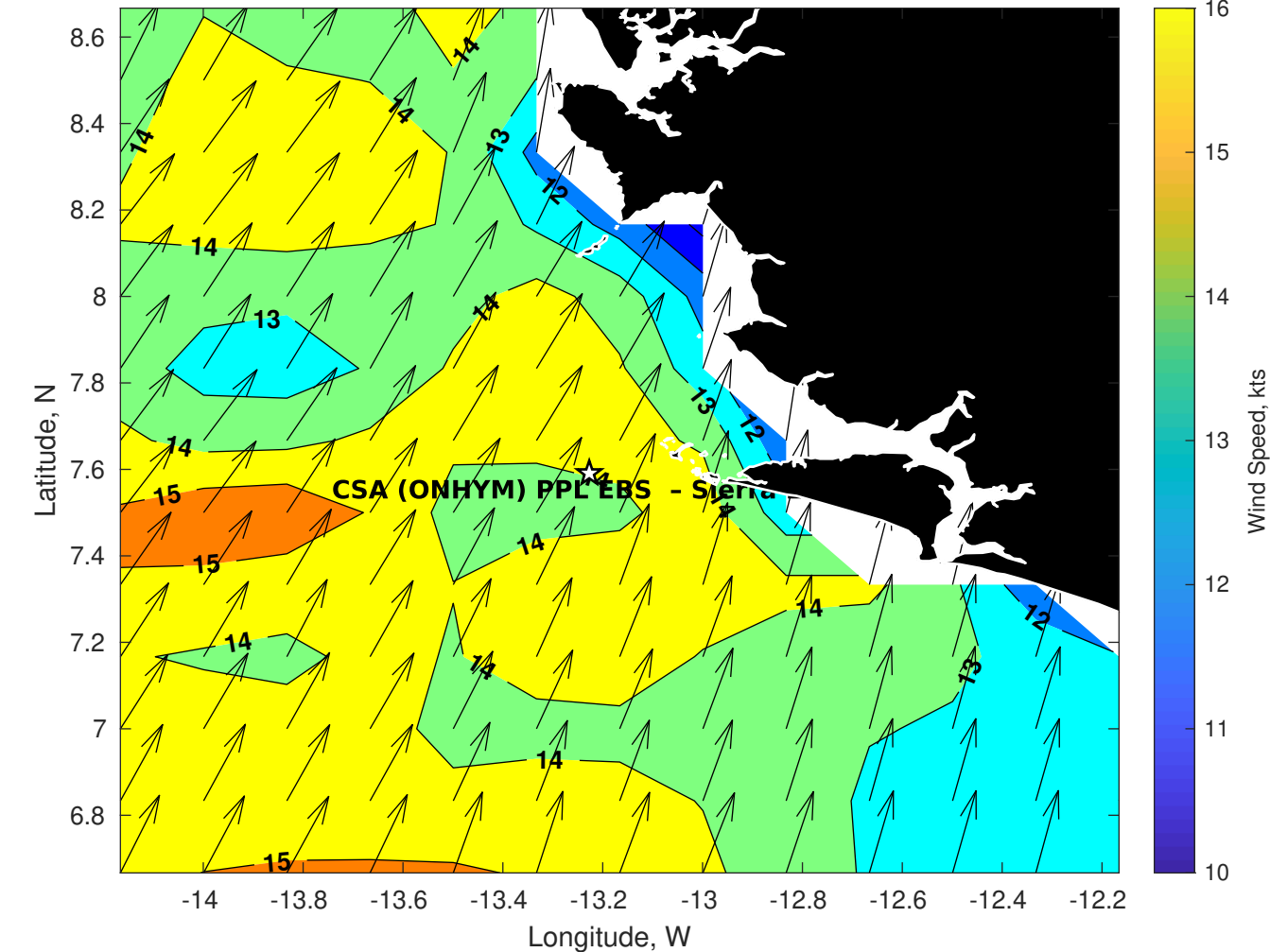
Winds (kts) for CSA (ONHYM) PPL EBS - Sierra Leone at 13-Aug-2025 09:00:00
