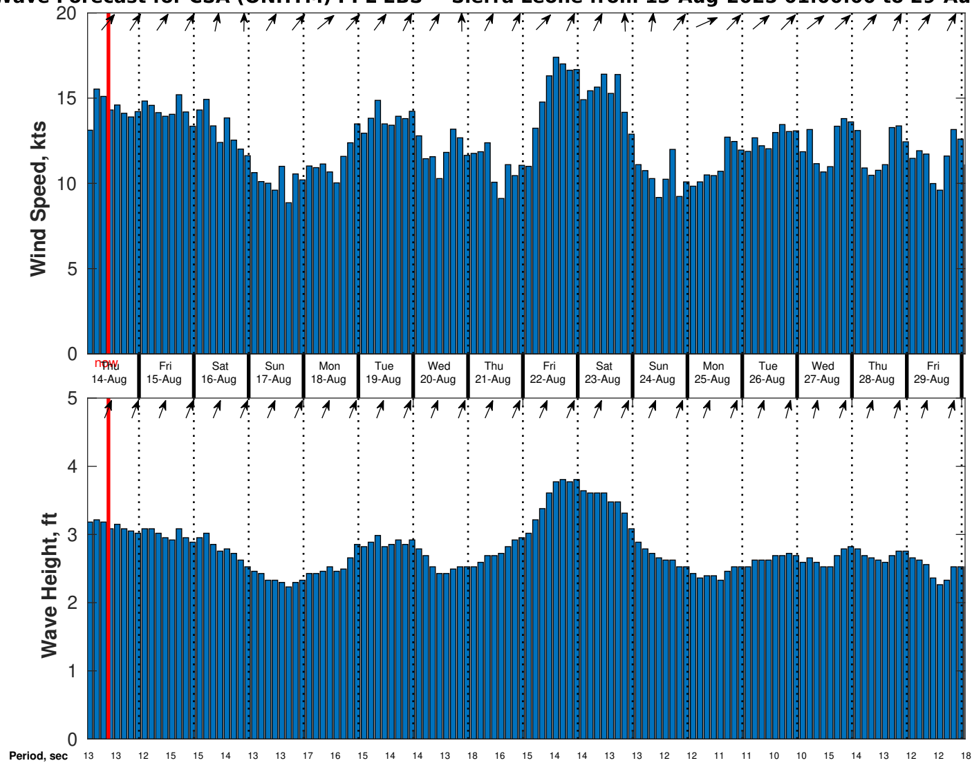
Wind & Wave Forecast for CSA (ONHYM) PPL EBS - Sierra Leone from 13-Aug-2025 01:00:00 to 29-Aug-2025 01:00:00
