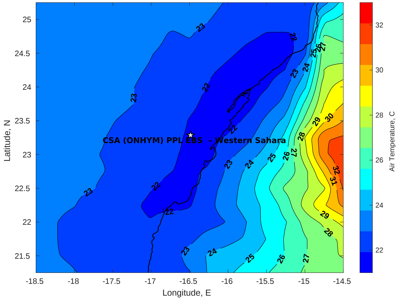
Air Temperature (C) for CSA (ONHYM) PPL EBS - Western Sahara at 13-Aug-2025
