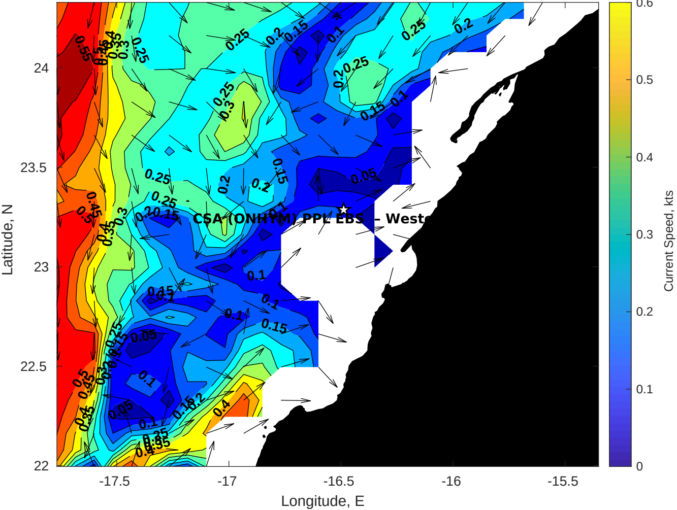
Surface Currents for CSA (ONHYM) PPL EBS - Western Sahara at 12-Aug-2025 00:00:00
