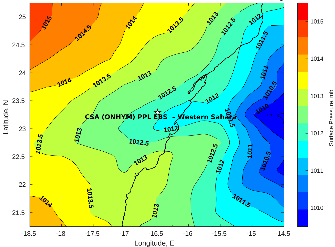
Surface Pressure (mb) for CSA (ONHYM) PPL EBS - Western Sahara at 15-Aug-2025 00:00:00
