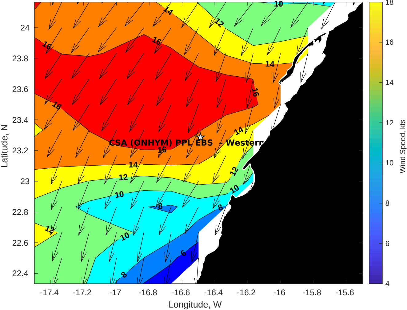
Winds (kts) for CSA (ONHYM) PPL EBS - Western Sahara at 13-Aug-2025 09:00:00
