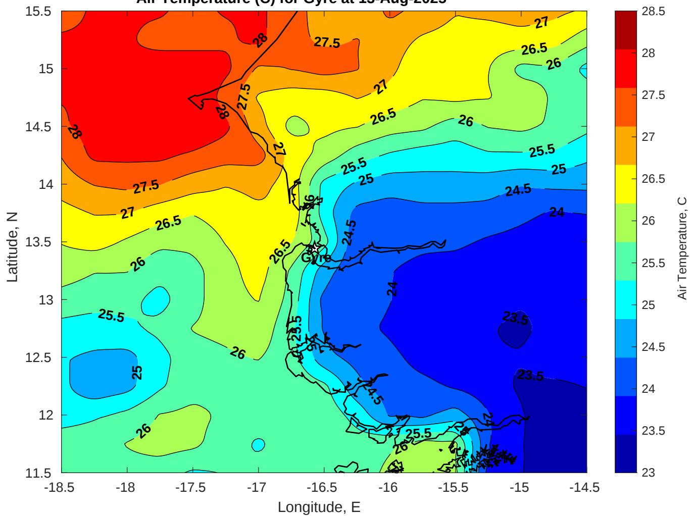
Air Temperature (C) for Gyre at 13-Aug-2025
