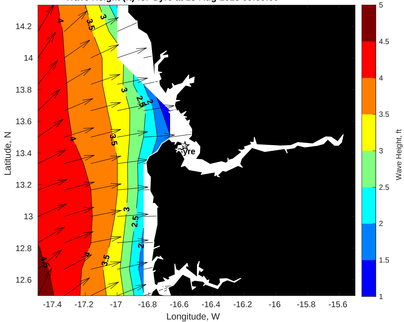
Wave Height (ft) for Gyre at 13-Aug-2025 09:00:00
