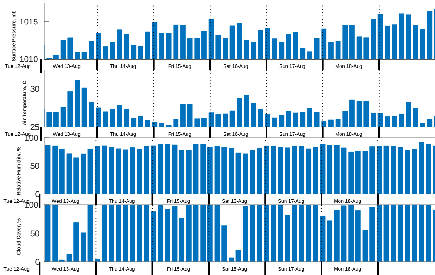
Met Forecast for Gyre from 12-Aug-2025 23:00:00 to 19-Aug-2025 23:00:00
