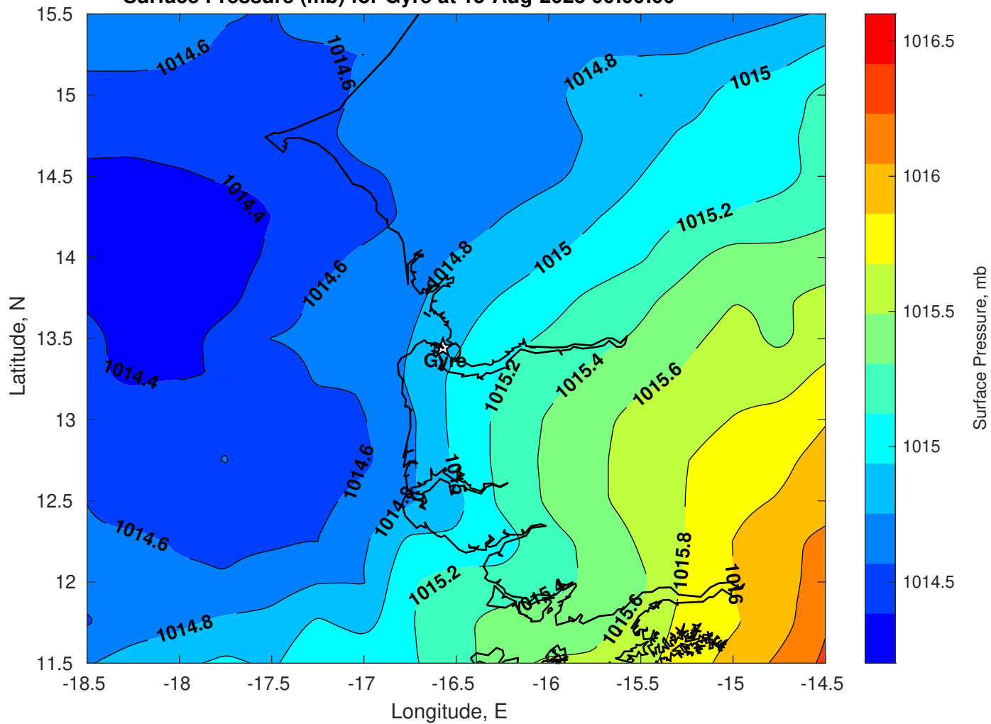
Surface Pressure (mb) for Gyre at 15-Aug-2025 00:00:00
