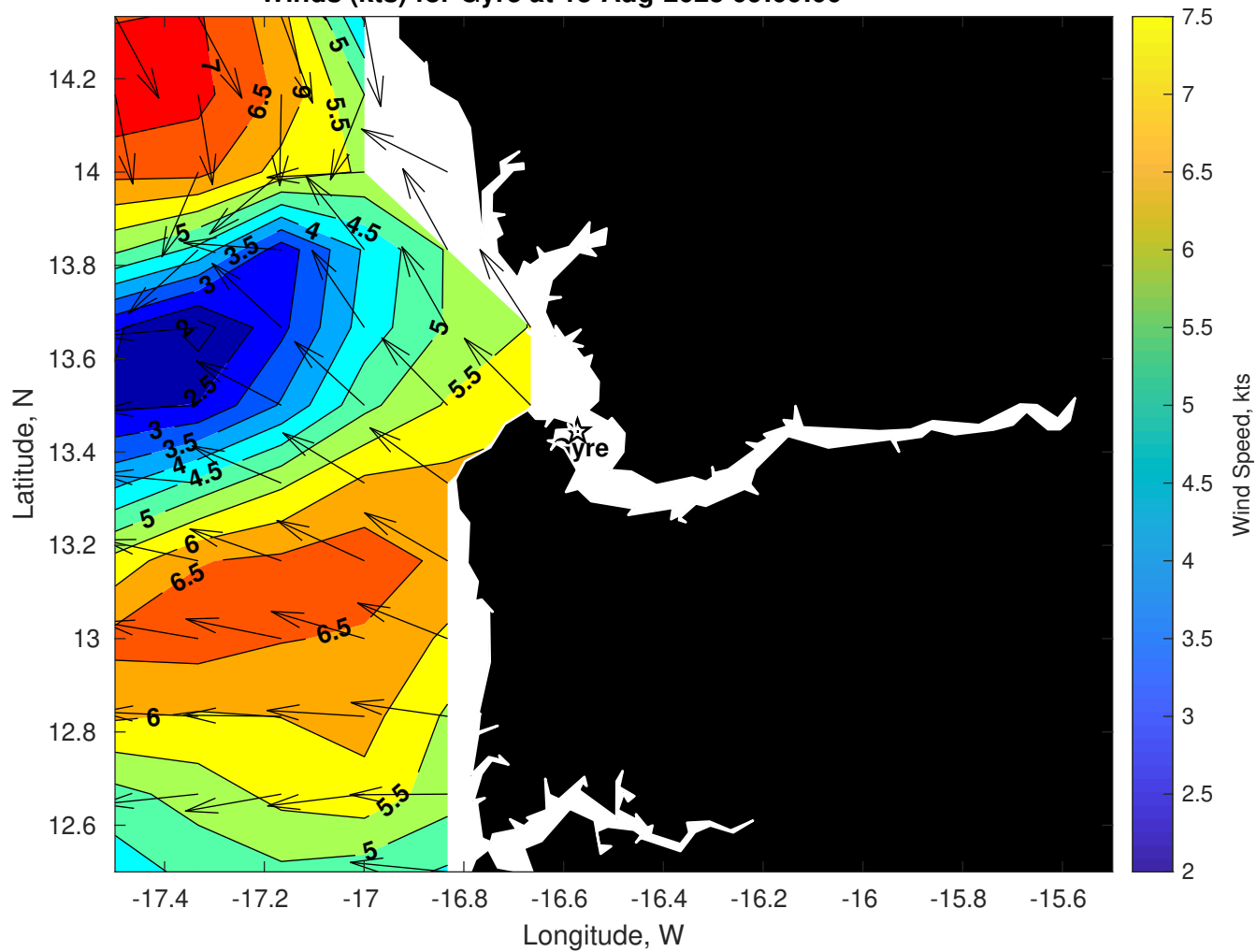
Winds (kts) for Gyre at 13-Aug-2025 09:00:00
