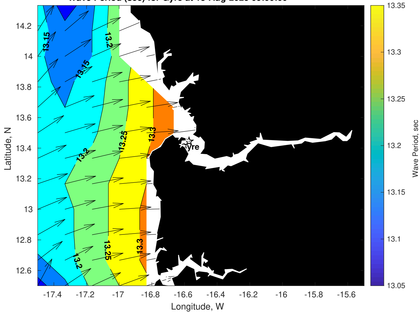
Wave Period (sec) for Gyre at 13-Aug-2025 09:00:00
