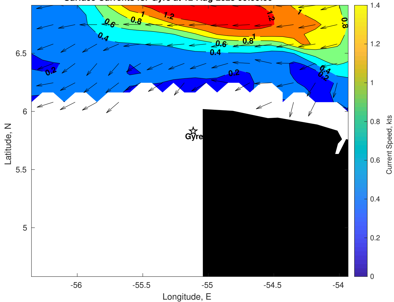
Surface Currents for Gyre at 12-Aug-2025 00:00:00
