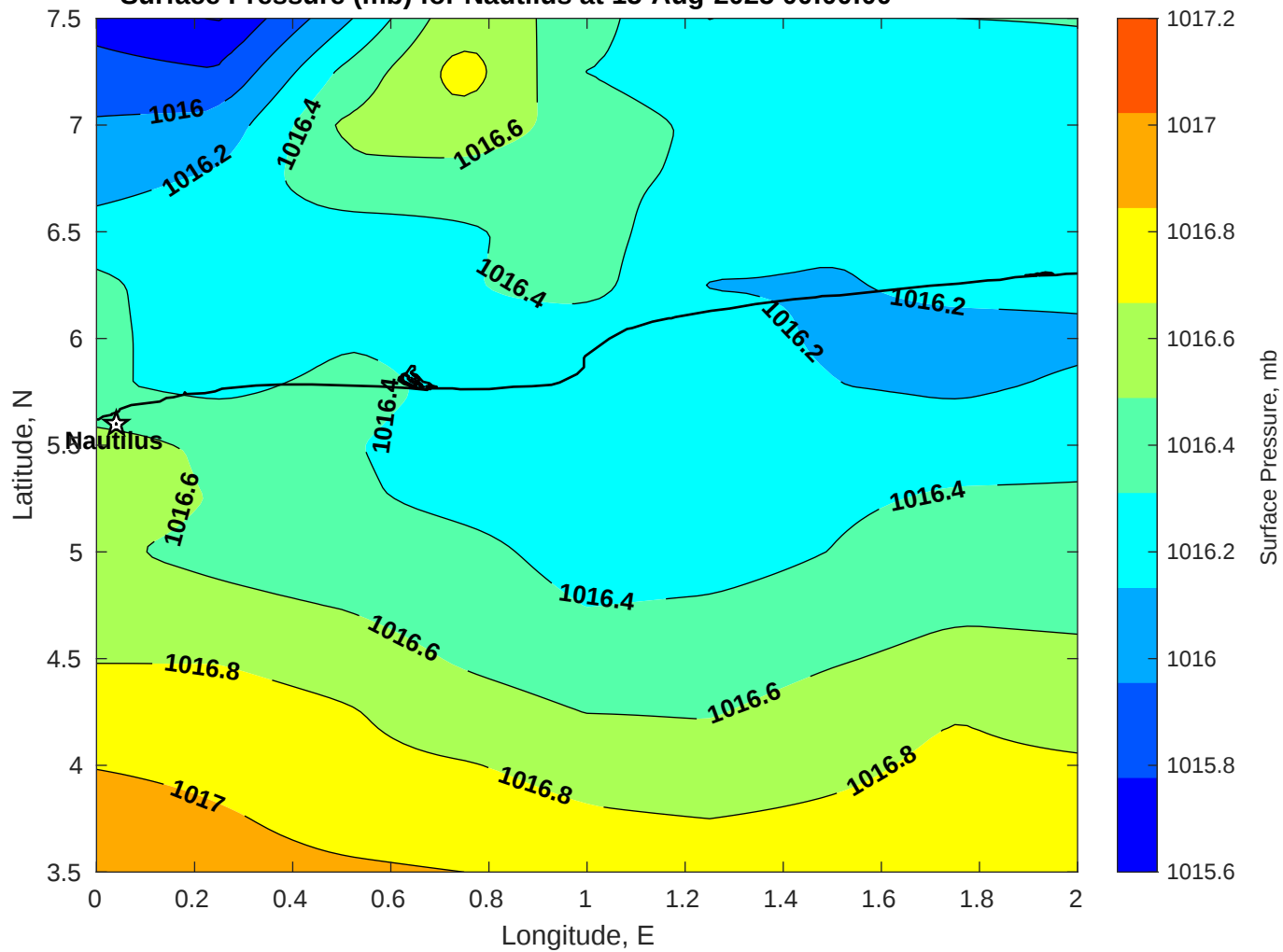
Surface Pressure (mb) for Nautilus at 15-Aug-2025 00:00:00
