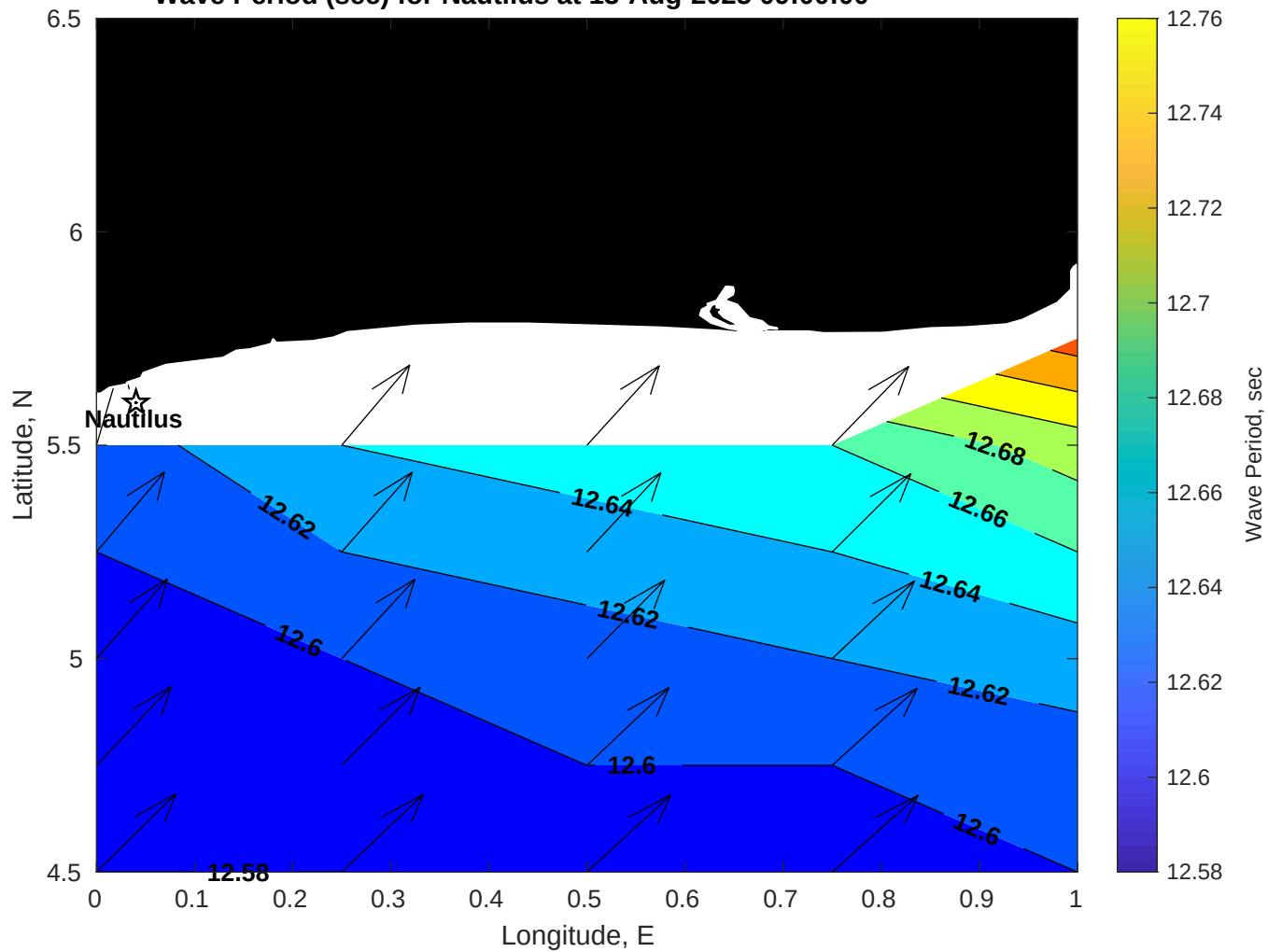
Wave Period (sec) for Nautilus at 13-Aug-2025 09:00:00
