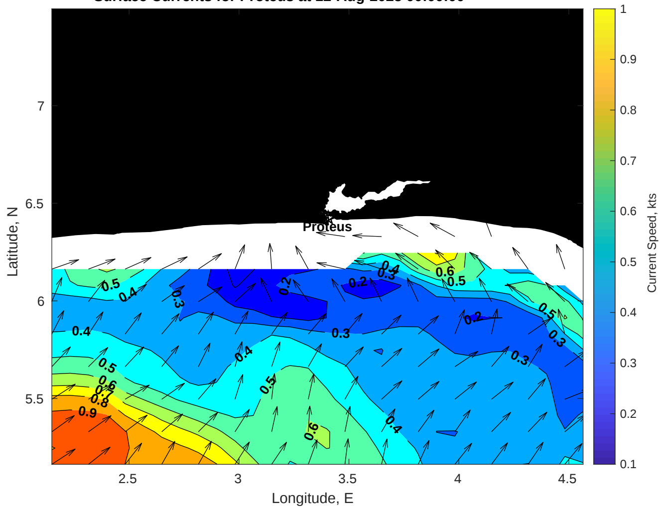
Surface Currents for Proteus at 12-Aug-2025 00:00:00
