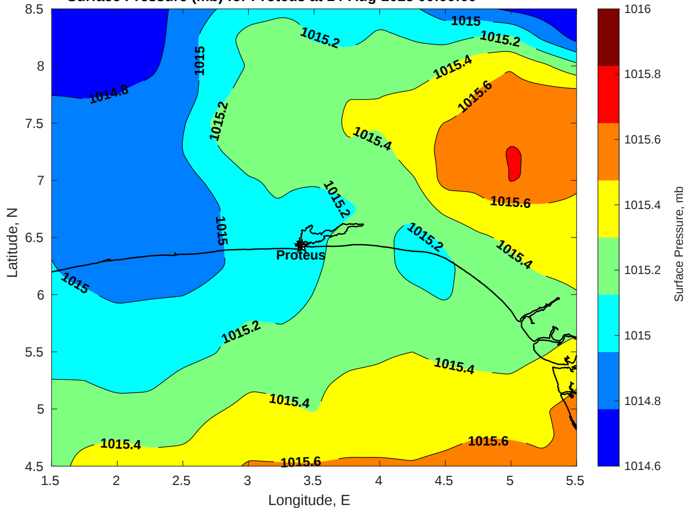
Surface Pressure (mb) for Proteus at 14-Aug-2025 00:00:00
