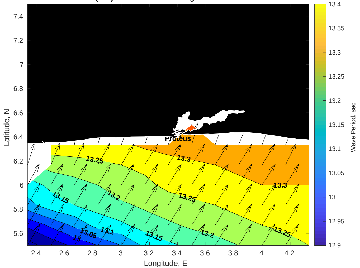
Wave Period (sec) for Proteus at 13-Aug-2025 09:00:00
