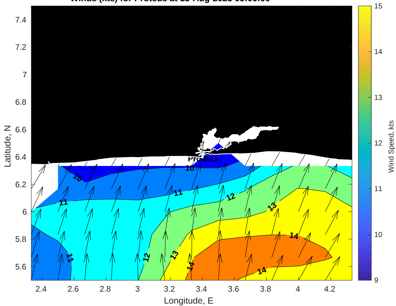
Winds (kts) for Proteus at 13-Aug-2025 09:00:00
