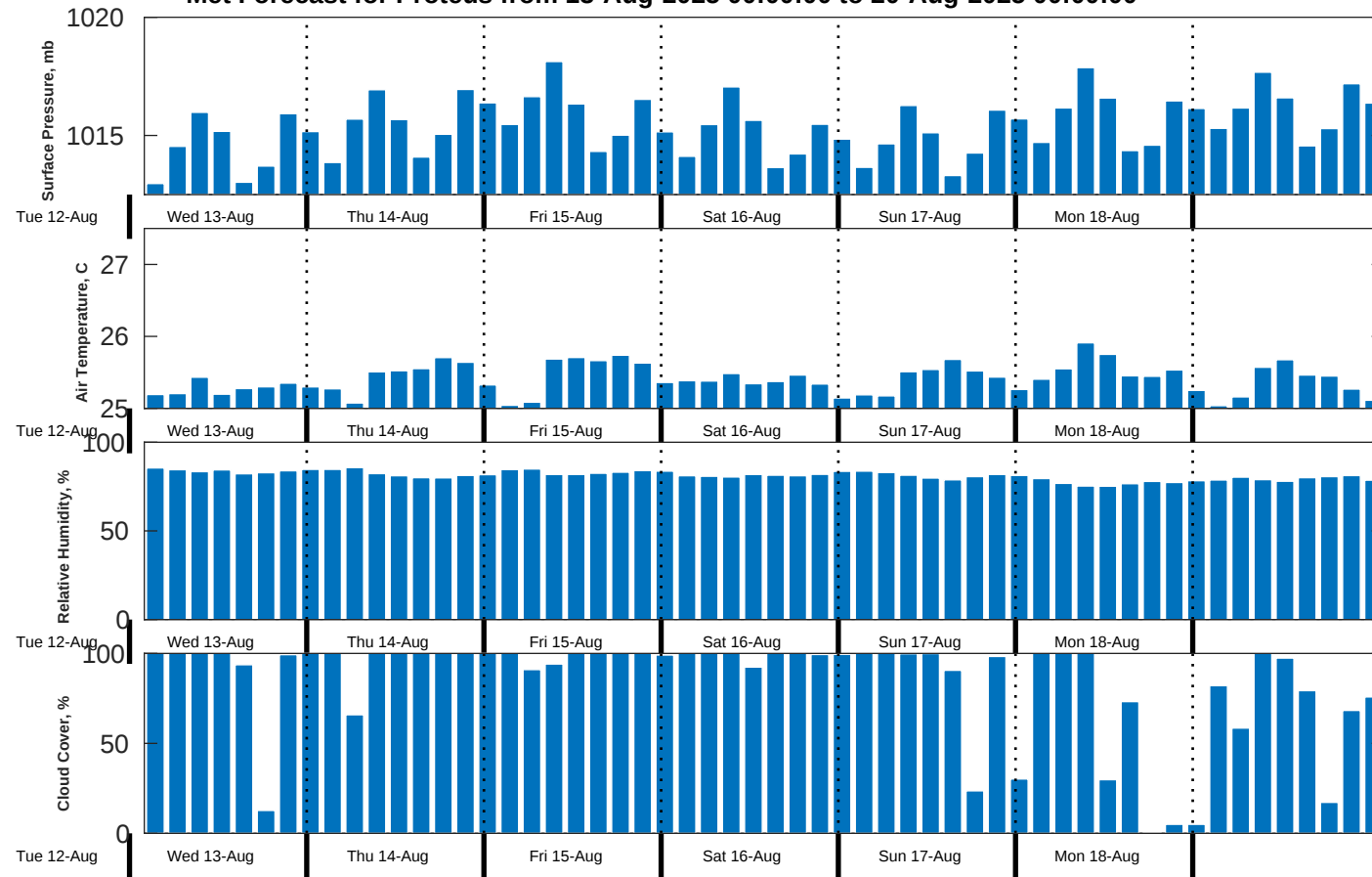
Met Forecast for Proteus from 13-Aug-2025 00:00:00 to 20-Aug-2025 00:00:00
