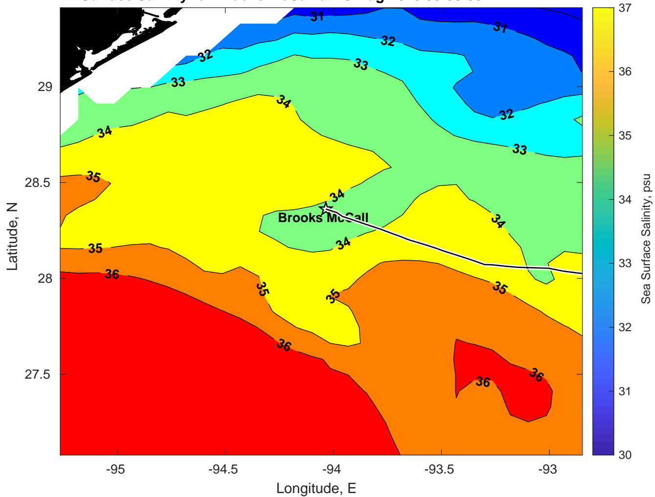
Surface Salinity for Brooks McCall at 13-Aug-2025 00:00:00
