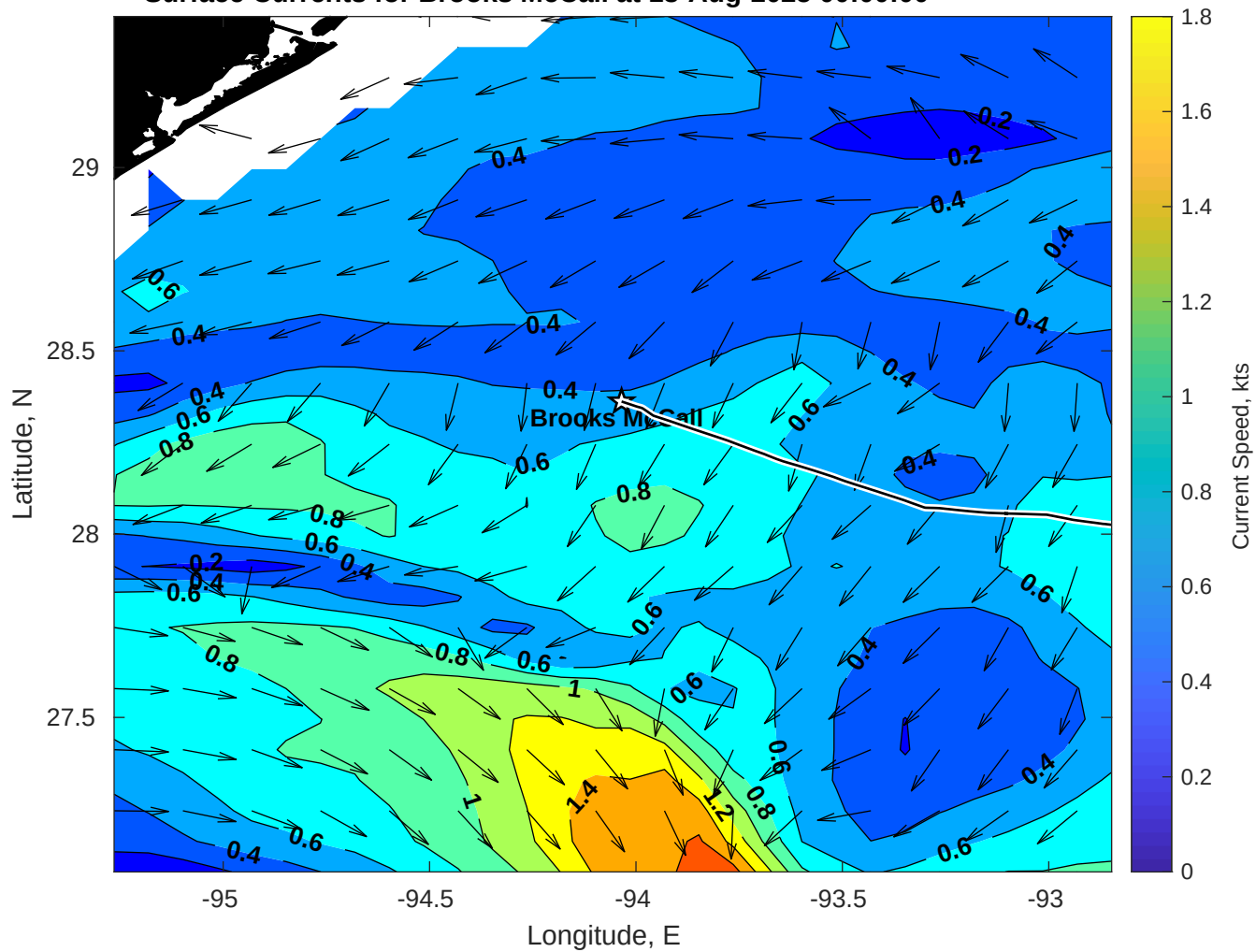
Surface Currents for Brooks McCall at 13-Aug-2025 00:00:00
