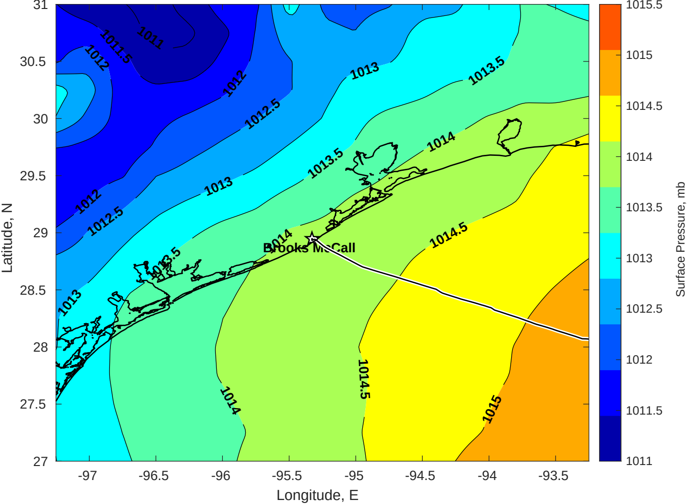
Surface Pressure (mb) for Brooks McCall at 15-Aug-2025 00:00:00
