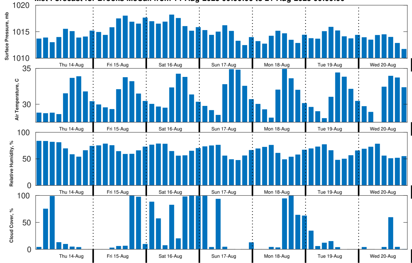
Met Forecast for Brooks McCall from 14-Aug-2025 00:00:00 to 21-Aug-2025 00:00:00
