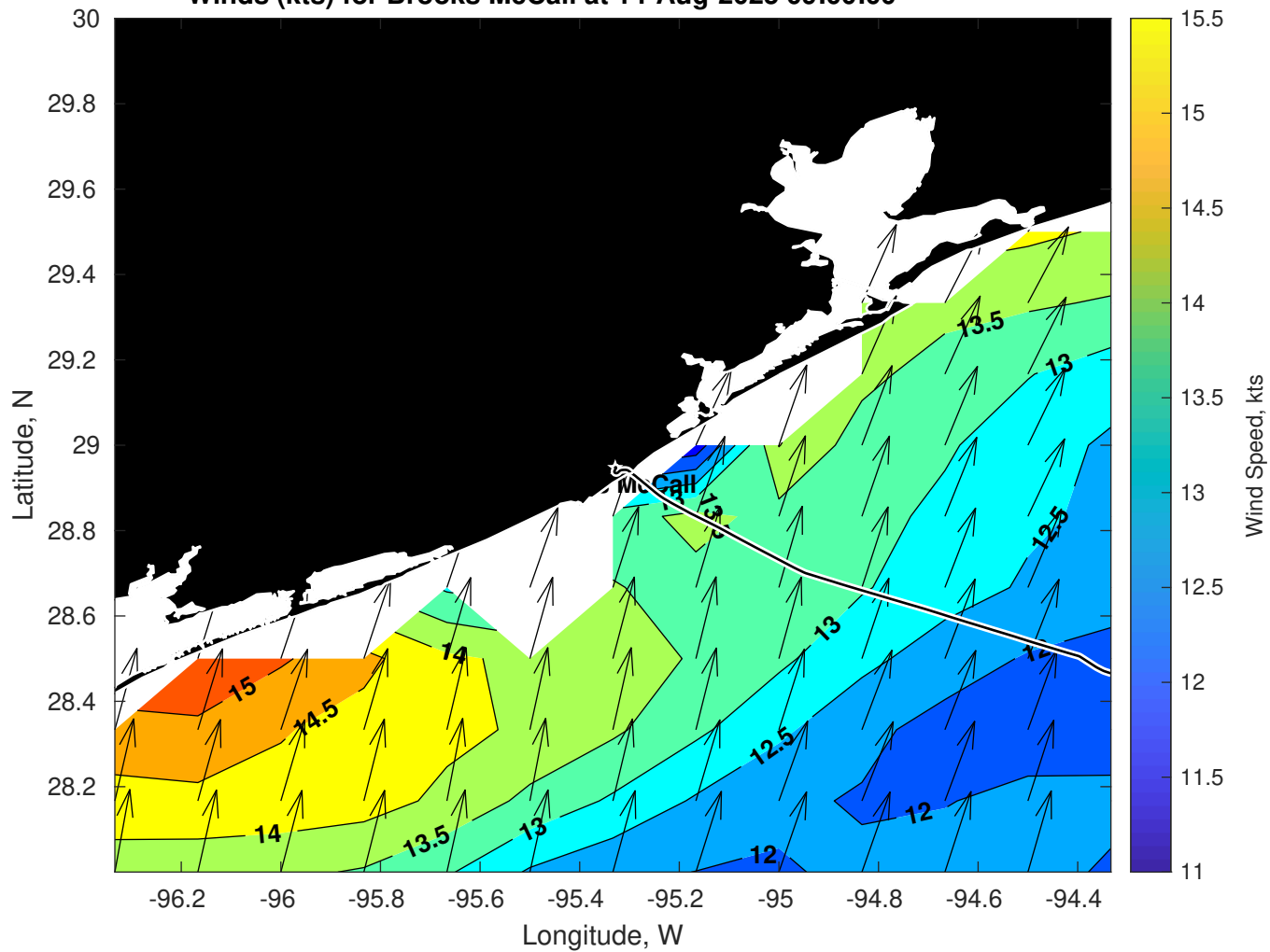
Winds (kts) for Brooks McCall at 14-Aug-2025 09:00:00
