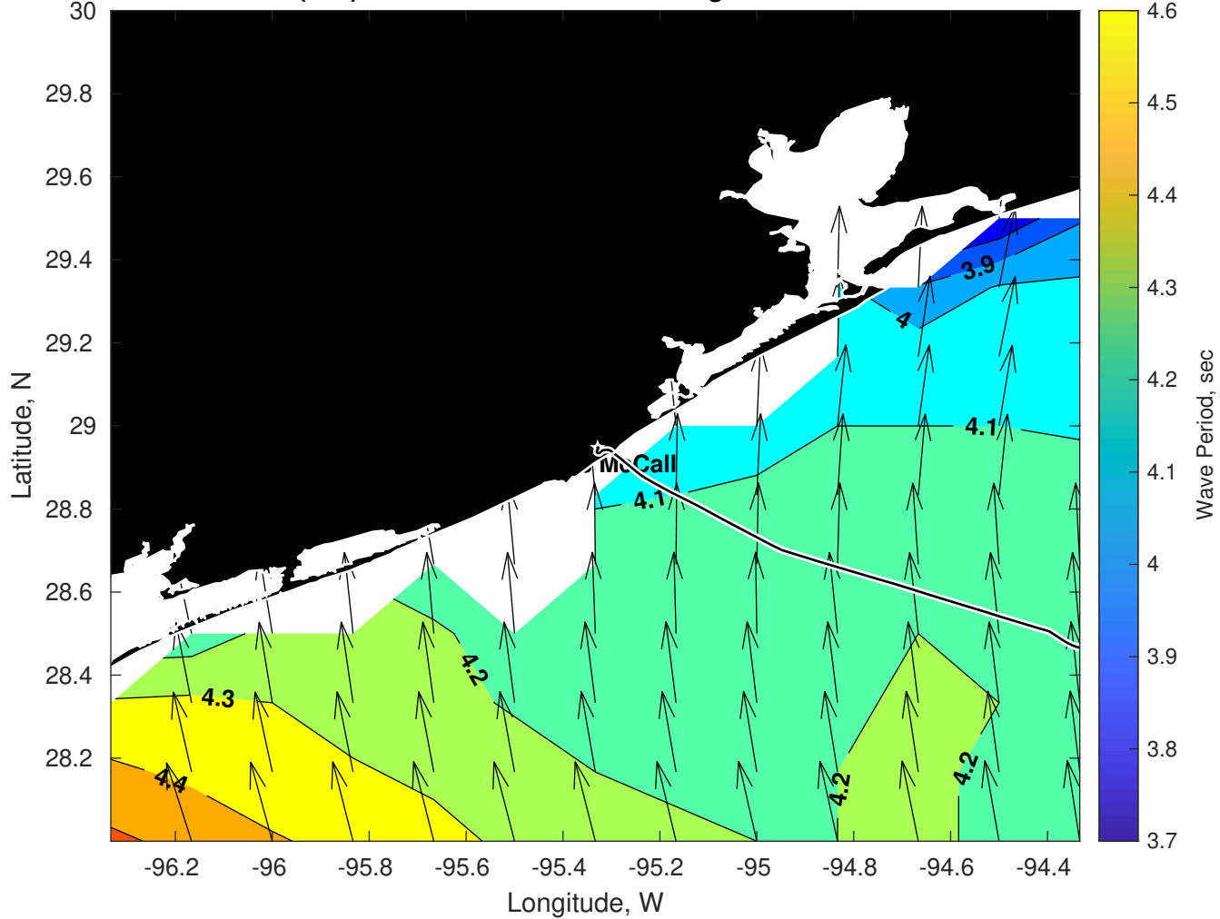
Wave Period (sec) for Brooks McCall at 14-Aug-2025 09:00:00
