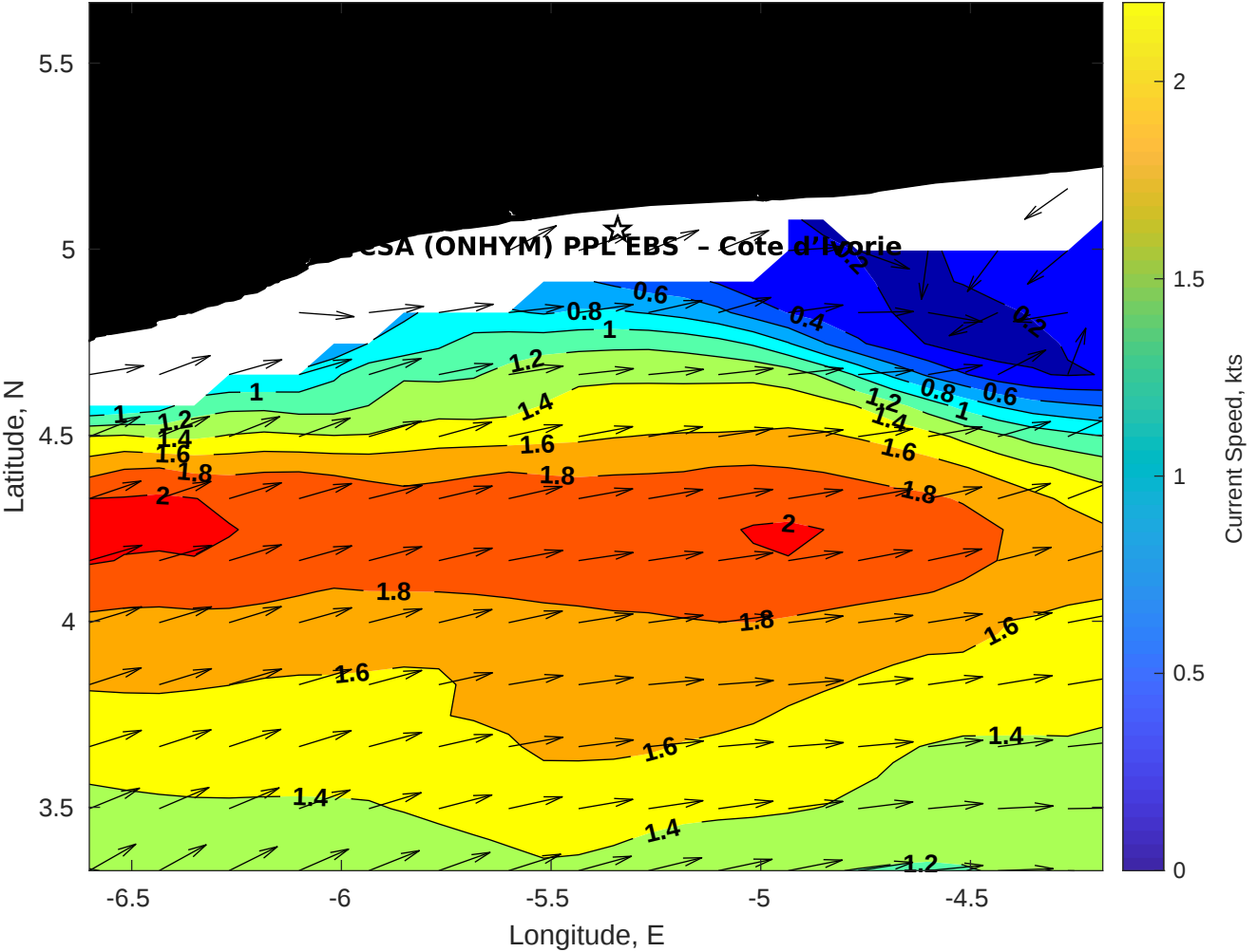
Surface Currents for CSA (ONHYM) PPL EBS - Cote d'Ivoire at 13-Aug-2025 00:00:00
