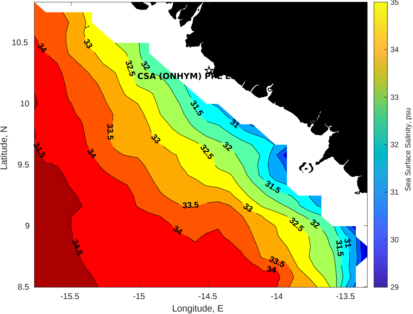
Surface Salinity for CSA (ONHYM) PPL EBS - Guinea at 13-Aug-2025 00:00:00
