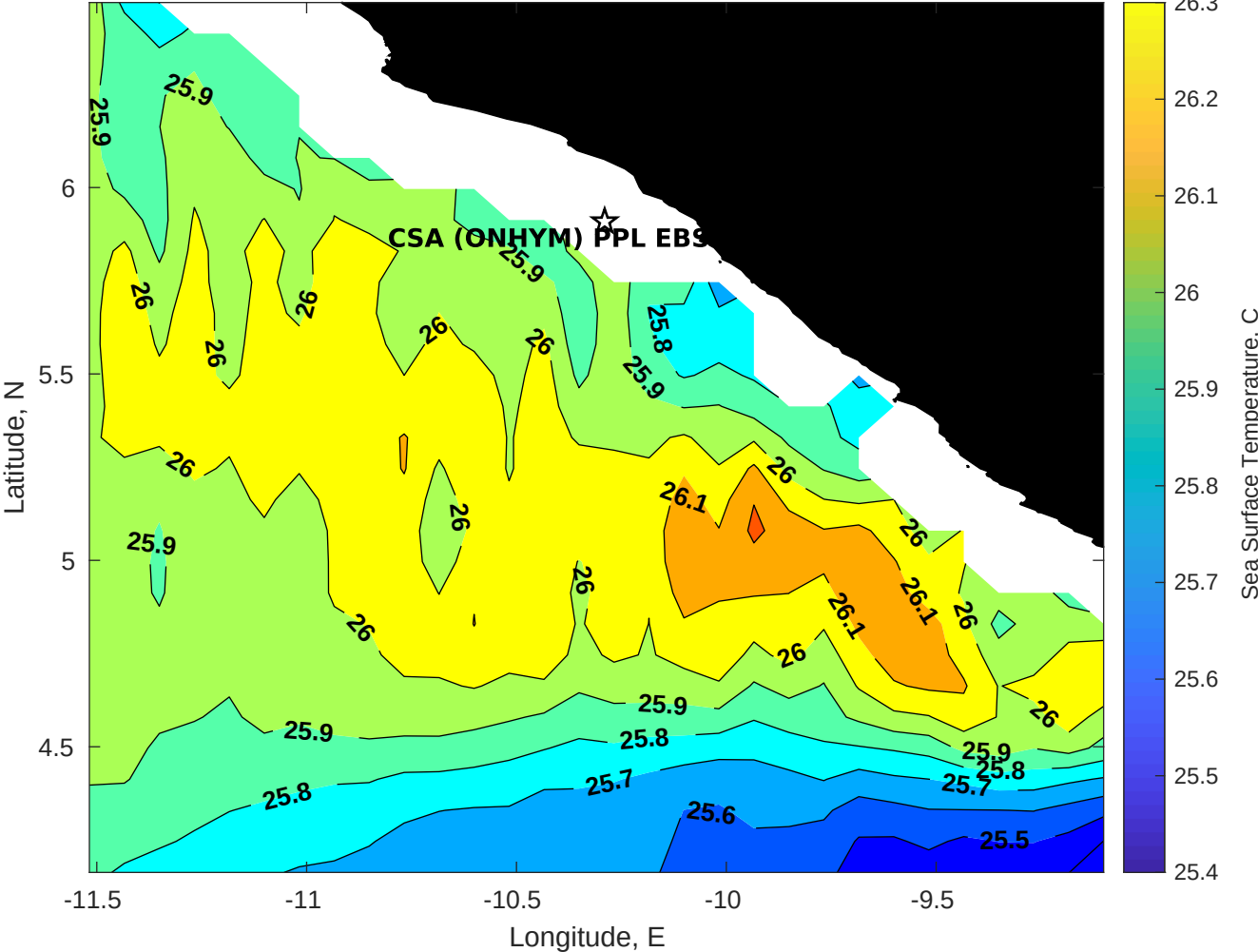
SST for CSA (ONHYM) PPL EBS - Liberia at 13-Aug-2025 00:00:00
